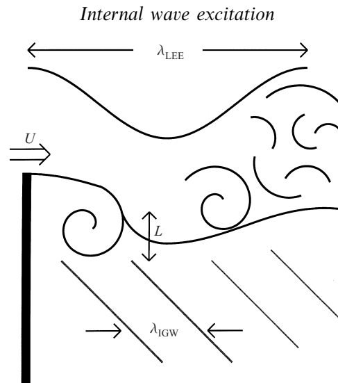
FIGURE 3. A schematic of the typical structure of the flow downstream of the barrier. The indicated length scale, L , and velocity scale U , are those relevant to the generation of IGW (of wavelength \lambda_{\text{IGW}} ) by vortices shed in the wake of the barrier. IGW excitation is distinct from the excitation of lee waves (of wavelength \lambda_{\text{LEE}} ), which develop on a scale U/N in which N is a characteristic value of the buoyancy frequency in the mixing region.
