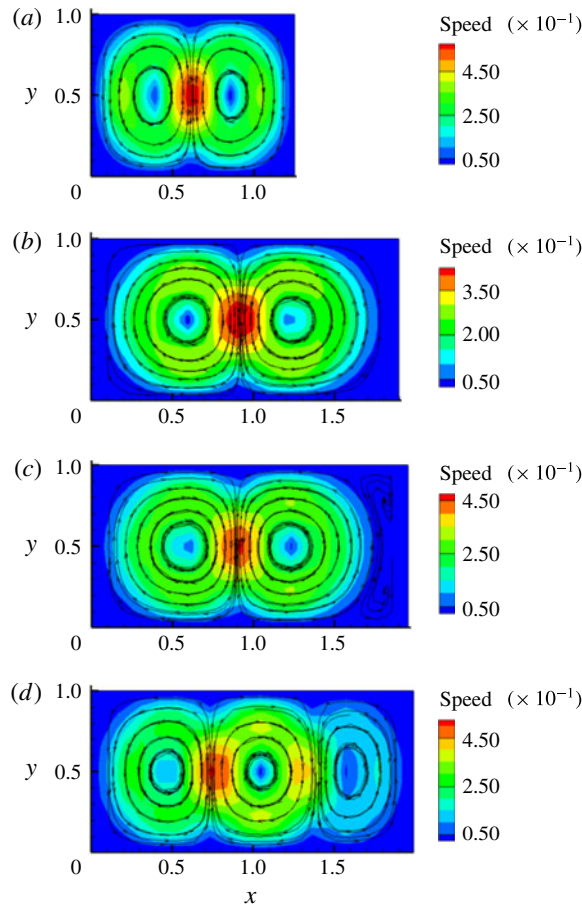
FIGURE 7. (Colour online) The flow pattern variation process as the film aspect ratio increases: (a) R=R_c=143.75 , \gamma=1.25 ; (b) R=R_c=121.43 , \gamma=1.89 ; (c) R=R_c=121.91 , \gamma=1.96 ; (d) R=R_c=121.67 , \gamma=1.99 .
