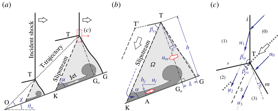
FIGURE 7. (Colour online) Schematics of the theoretical model showing (a) the self-similar flow of Mach reflection, (b) an enlarged view of the control body and (c) the pseudo-steady flow in the vicinity of and with respect to the triple point.
