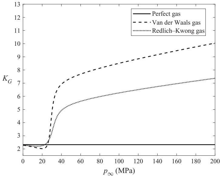
Figure 18. Thermodynamic similarity parameter K_G as a function of p_\infty at T_\infty = 700 K for different gas models.
