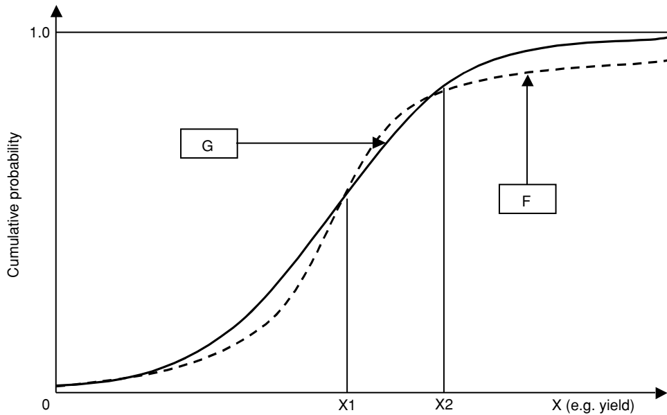
Figure 2. Example of Second-Degree Stochastic Dominance (F dominates G in SSD). See text for explanation of variables.
