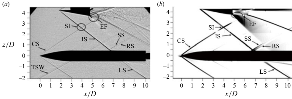
Figure 25. Comparison of flow field structures between the CFD and experiment: (a) experiment result; (b) CFD result. Shock-shock intersection (SI), expansion fan (EF), conical shock (CS), incident shock (IS), separation shock (SS), reattachment shock (RS), test section Mach wave (TSW), leeward shock (LS).
