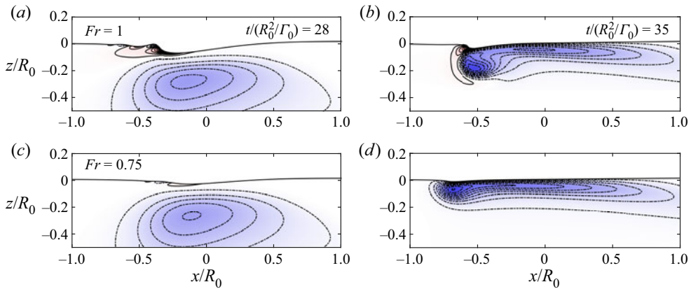
Figure 38. Contours of spanwise vorticity ( \omega_y ) in the symmetry plane, at flow times (a,c) t/(R_0^2/\Gamma_0) = 28 and (b,d) t/(R_0^2/\Gamma_0) = 35 , and at Froude numbers (a,b) Fr = 1 and (c,d) Fr = 0.75 , obtained using the moving-mesh solver (interTrackFoam). The contour levels and colourmap are the same as in figure 19. The physical parameters are Re = 1570 , \alpha = 80^\circ , a/R_0 = 0.35 and H/R_0 = 2.5
