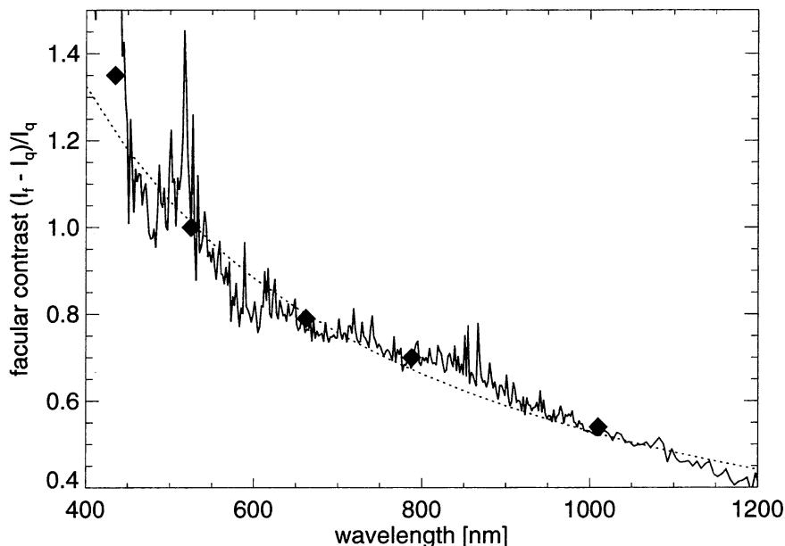
Figure 2. Intensity contrast of faculae vs. wavelength. Observational results are indicated by the filled diamonds, the model predictions by the solid curve. The plotted values correspond to \mu = 0.25 , where \mu is the heliocentric angle (from Unruh et al. 1999).
