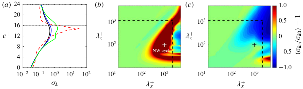
FIGURE 9. (a) Singular values for the non-rotating (black line) and rotating cases (coloured lines) at Re_\tau = 2000 . Blue line, Ro_\tau/Re_\tau = 5.5 \times 10^{-4} ; green line, Ro_\tau/Re_\tau = 2.5 \times 10^{-3} ; red line, Ro_\tau/Re_\tau = 1.6 \times 10^{-2} . The figure considers modes with length scales comparable to the NW cycle. (b,c) Singular value ratios as a function of streamwise and spanwise wavelength at Ro_{\tau,2000} = 3.3 \times 10^1 ( Ro_\tau/Re_\tau = 1.6 \times 10^{-2} ): (b) integrated over wave speed 0 \leq c^+ < 16 ; (c) integrated over wave speed 16 \leq c^+ \leq U_{CL}^+ .
