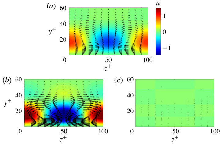
FIGURE 5. Singular value-weighted velocity structure for NW modes at Re_\tau = 180 : (a) non-rotating; (b) Ro_{\tau,180} = 1 ; (c) Ro_{\tau,180} = 40 . Velocities are normalized by the maximum value in the non-rotating case.
