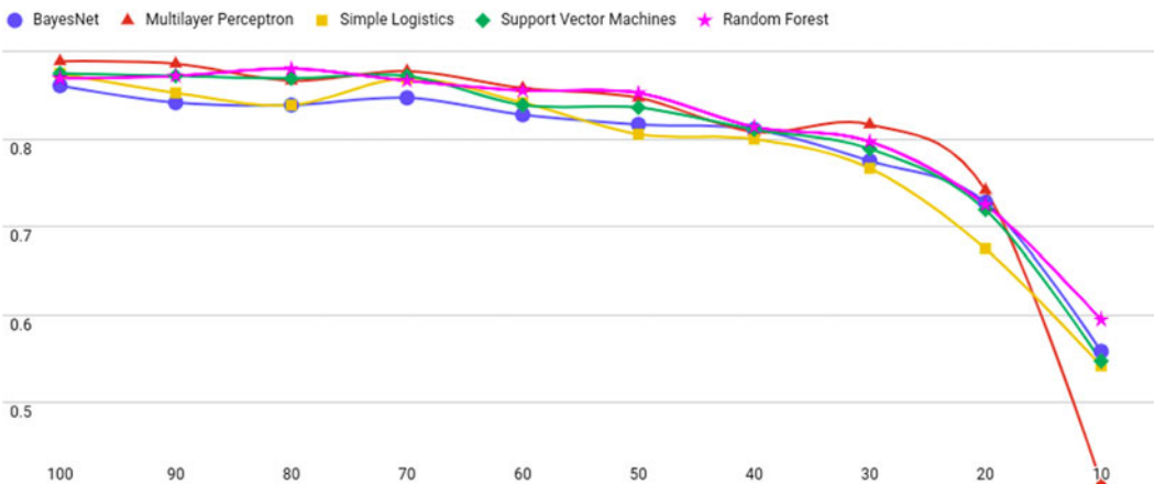
Figure 14. Accuracy when the number of tweets per user decreases (ARAP-Tweet corpus).
