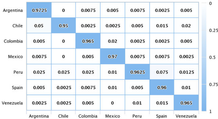
Figure 6. Confusion matrix for Spanish varieties for LDSE on the PAN-AP'17 corpus.
