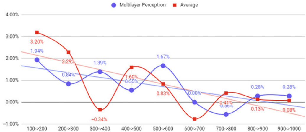
Figure 13. Accuracy improvement for each increment in the number of tweets per user in steps of 100 (ARAP-Tweet corpus).
