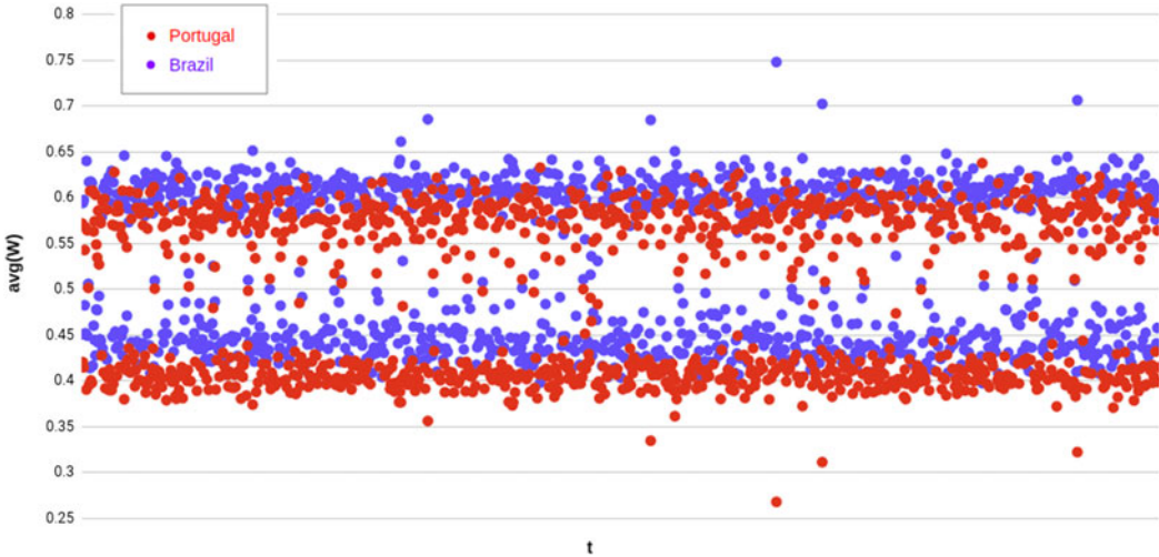
Figure 1. Portuguese subset of the PAN-AP'17 represented with the avg(W) feature of LDSE. The x-axis represents each of the terms in the corpus. The Y-axis represents the average weight for each term in Brazilian (blue) or Portuguese (red) varieties.
