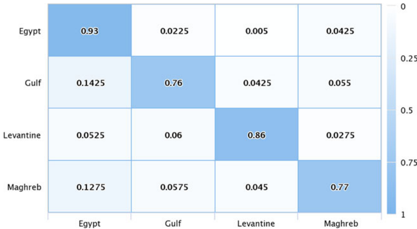
Figure 3. Confusion matrix for Arabic varieties with LDSE on the PAN-AP'17 corpus.
