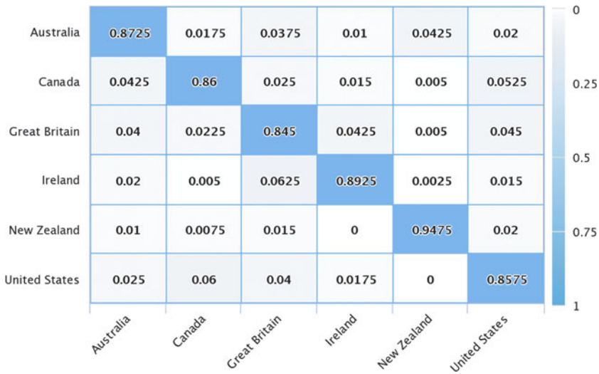
Figure 4. Confusion matrix for English varieties for LDSE on the PAN-AP'17 corpus.
