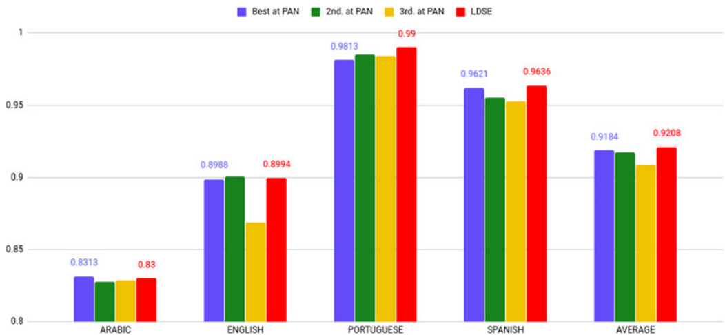
Figure 2. Comparative results of the three best performing teams in the Author Profiling shared task at PAN 2017 versus LDSE. The best performing team (Basile et al. 2017) obtained the highest result in Arabic and Spanish. The second best performing team (Tellez et al. 2017) obtained the highest result in English and Portuguese.
