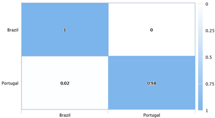
Figure 5. Confusion matrix for Portuguese varieties for LDSE on the PAN-AP'17 corpus.
