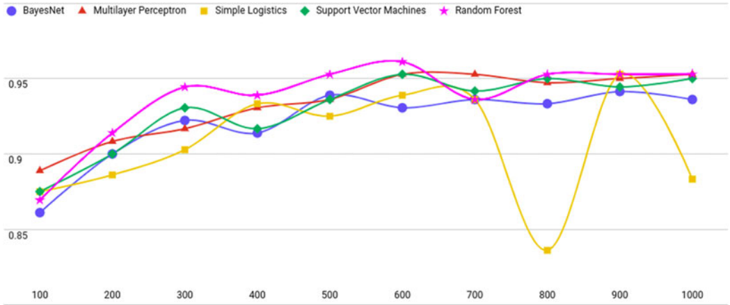
Figure 12. Accuracy when the number of tweets increases (ARAP-Tweet corpus).
