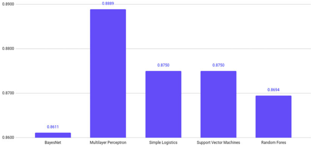
Figure 8. Accuracy obtained by LDSE with five different machine learning classifiers on the ARAP-Tweet corpus.
