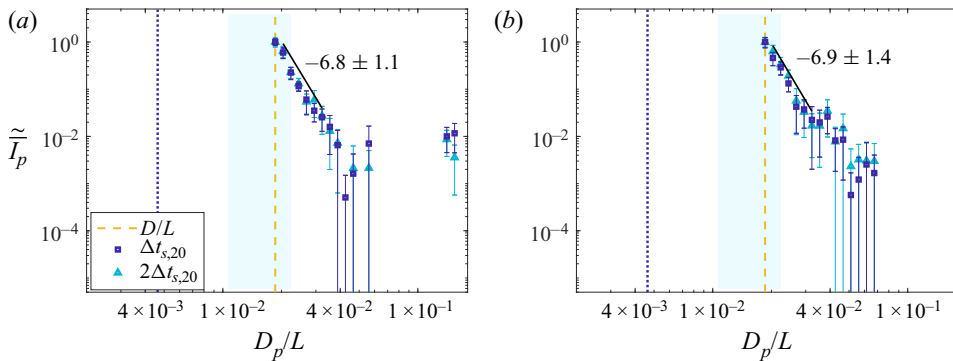
Figure 13. The normalized differential incoming transfer rate \tilde{I}_p^T(D_{p,j}; t|D) from parent bubbles as a function of non-dimensional parent bubble size D_p/L for the 20-realization baseline ensemble subset at the non-dimensional cutoff size D/L = 1.86 \times 10^{-2} , and at the times (a) t = 2.51 and (b) t = 2.99 . These statistics are averaged over the non-dimensional sampling interval 16\Delta t_{s,20} = 9.6 \times 10^{-2} used in figure 8. For a description of the normalization, shaded regions, vertical lines, excluded events, error bars, bubble-size subrange and dataset for the power-law fits, and the fit-exponent uncertainties, refer to the caption of figure 12.
