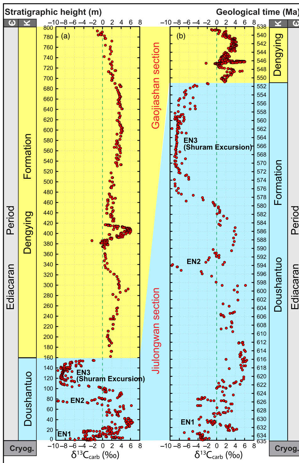
Fig. 15. (Colour online) \delta^{13}\text{C}_{\text{carb}} (‰, VPDB) chemostratigraphic data for the Ediacaran Period in South China plotted against (a) stratigraphic height and (b) estimated geological time. Data sources: Doushantuo Formation at the Jiulongwan section (Jiang et al. 2007; McFadden et al. 2008); Dengying Formation at the Gaojiashan section (H. Cui, unpub. Ph.D. thesis, Univ. Maryland, 2015; Cui et al. 2016b). Abbreviations: K – Kuanchuanpu Formation; \epsilon – Cambrian; Cryog. – Crogenian Period; EN – Ediacaran \delta^{13}\text{C}_{\text{carb}} negative excursions. See the main text for detailed discussion.
