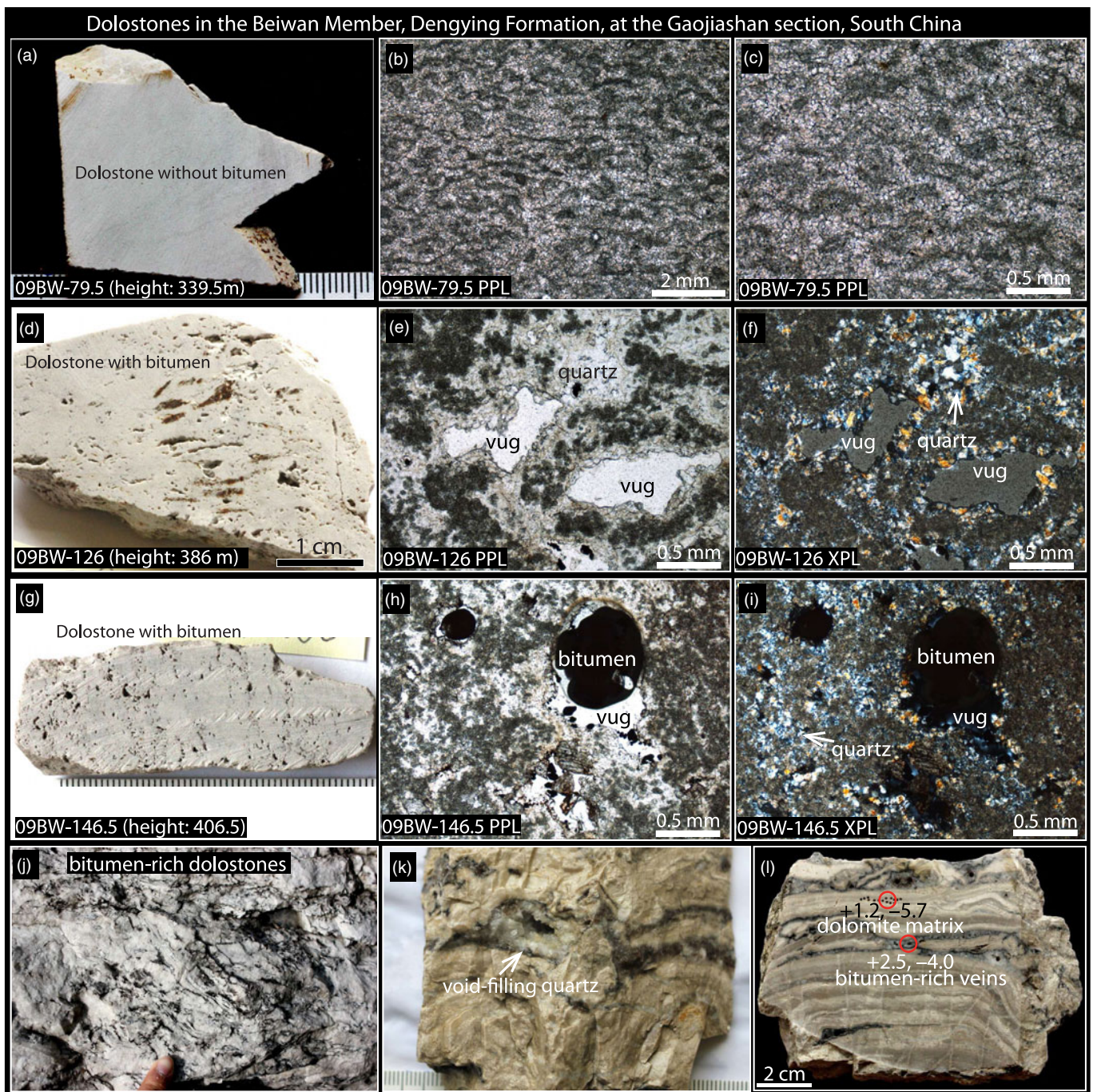
Fig. 8. (Colour online) Petrographic observations of dolostones in the Beiwang Member, Dengying Formation, at the Gaojiashan section. (a–c) Slab and petrographic photographs of sample 09BW-79.5 (collected at 339.5 m in Fig. 12) showing dolomicrite with abundant algal fabrics (?). (d–f) Slab and petrographic photographs of sample 09BW-126 (collected at 386 m in Fig. 12) showing dolostone with vugs and quartz cements. (g–i) Slab and petrographic photographs of sample 09BW-146.5 (collected at 406.5 m in Fig. 12). Note the vugs with bitumen in (h) and (i), and the quartz cements (arrows) in (f) and (i) under cross-polarized light. (j) Outcrop photograph showing dolostones (white) with abundant bitumen (black). (k, l) Photographs of hand samples showing bitumen in dissolution vugs. Note the void-filling quartz (arrow) in (k). Micro-drilling geochemical \delta^{13}\text{C} (left) and \delta^{18}\text{O} (right) data are provided in (l). PPL – plane polarized light; XPL – cross-polarized light.
