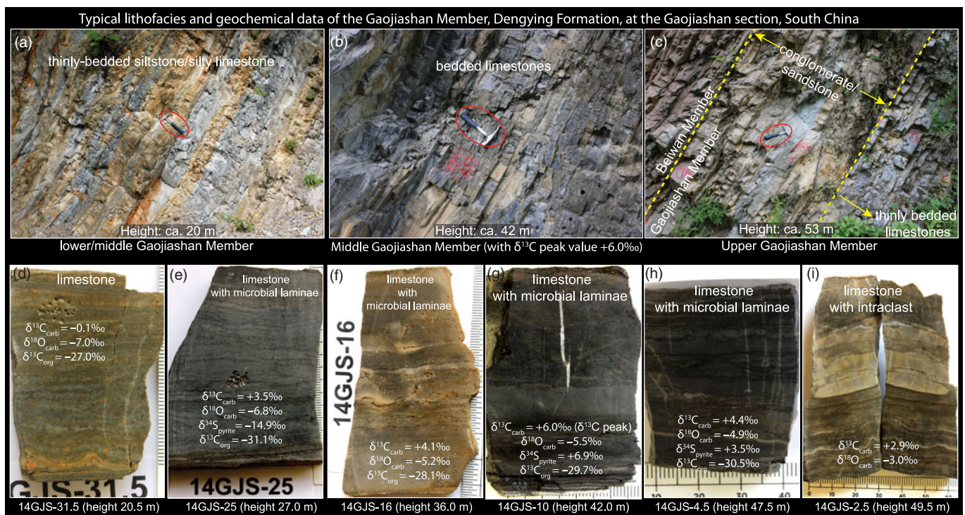
Fig. 6. (Colour online) Typical lithofacies and geochemical data of the Gaojiashan Member, Dengying Formation, at the Gaojiashan section. Stratigraphic height numbers represent the distance above the Algal Dolomite/Gaojiashan boundary. (a) Thinly bedded siltstones and silty limestones in the lower/middle transition of the Gaojiashan Member. (b) Dark-coloured thin-bedded limestones in the middle Gaojiashan Member that records a \delta^{13}\text{C}_{\text{carb}} positive excursion of up to +6‰ (Cui et al. 2016b). (c) A conglomerate/sandstone interval in the upper Gaojiashan Member. Hammer for scale is 33 cm long. (d–i) Photographs of freshly cut slabs of samples from the Gaojiashan Member with microbial laminae and intraclasts. These slabs represent (d) greenish grey dolostone, (e–h) limestones with microbial laminae, and (i) intraclastic limestone. The numbers in the sample IDs represent distance (in metres) below the conglomerate interval in the upper Gaojiashan Member; for example, sample 14GJS-10 is 10 m below the conglomerate interval in the Gaojiashan Member. The \delta^{13}\text{C}_{\text{carb}} and \delta^{18}\text{O}_{\text{carb}} values of micro-drilled carbonate powders are marked on the slab. The \delta^{34}\text{S}_{\text{pyrite}} and \delta^{13}\text{C}_{\text{org}} values of each slab were analysed from bulk acidified residues.
