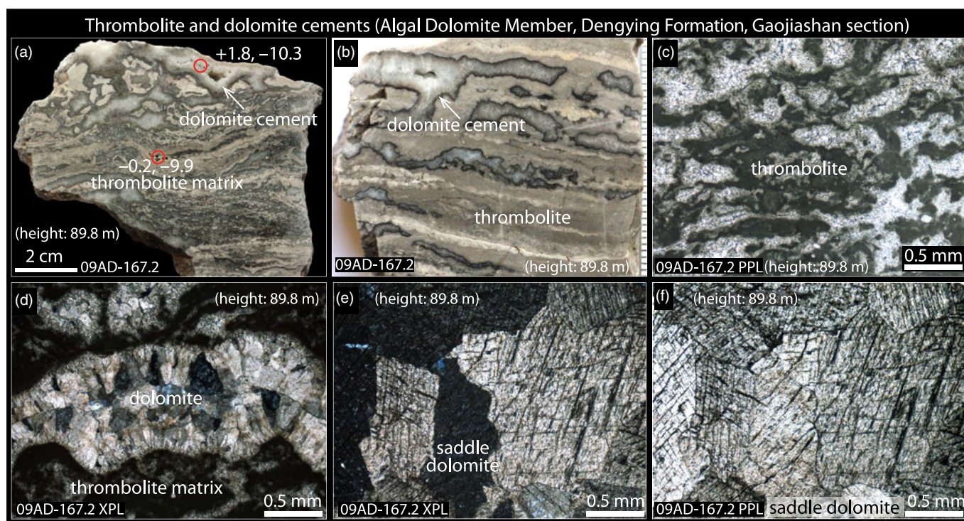
Fig. 5. (Colour online) Thrombolitic dolostone and void-filling hydrothermal dolomite cements in the Algal Dolomite Member, Dengying Formation, at the Gaojiashan section. Sample 09AD-167.2 from a stratigraphic height of 89.8 m in Figure 12. (a, b) Dolostone slabs showing thrombolitic dolomite matrix with vug-filling dolomite cements. Fabric-specific \delta^{13}\text{C} (left) and \delta^{18}\text{O} (right) data are provided in (a). Scale in (b) in millimetres. (c) A magnified view of the thrombolitic dolomite matrix under plane-polarized light. (d) A magnified view of coarse dolomite cements in the thrombolitic dolomite matrix under cross-polarized light. (e, f) Magnified views of hydrothermal saddle dolomites with two distinct sets of cleavages and sweeping extinction. PPL – plane polarized light; XPL – cross-polarized light.
