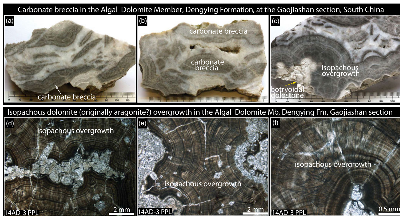
Fig. 3. (Colour online) Field samples and microscopic views of the carbonate breccia and isopachous overgrowth that are typical in the lower half of the Algal Dolomite Member of the Dengying Formation at the Gaojiashan section. (a–c) Karst breccia cemented by carbonates in the vugs between breccias. Scale in millimetres. (d–f) Petrographic images of sample 14AD-3, showing isopachous void-filling carbonate cements with concentric textures (brown colour) surrounding coarse dolomite sediments (white colour). PPL – plane polarized light.
