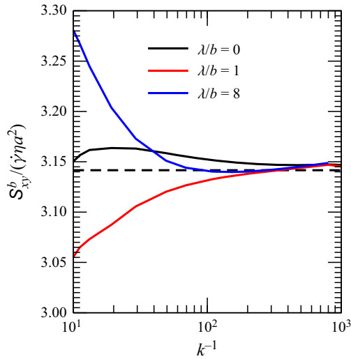
Figure 8. Value of S_{xy}^b vs k for \lambda/b = 0, 1 and 8 . Dashed line: analytical prediction given in (3.22).
