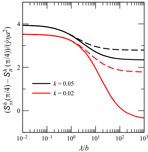
Figure 6. Value of S_{ss}^h(\pi/4) - S_{tt}^h(\pi/4) vs \lambda/b . Comparison of numerical solution of the boundary integral equation given in (2.4) for (i) the full version (full lines) and (ii) the leading-order approximation for small k as given in (3.17) and (3.18) (dashed line).
