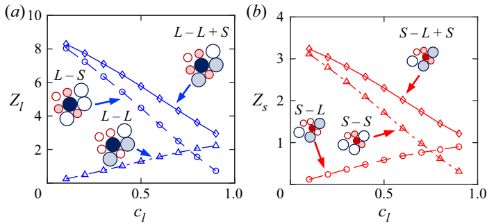
Figure 5. Dependence of coordination number Z_i for (a) large and (b) small particles on large-particle concentration for size ratio d_l/d_s = 2 . Z_i for large or small particles (solid curve) can be separated into same-species (dash-dot) and interspecies (dashed) coordination numbers depending on the species of the contacting particles.
