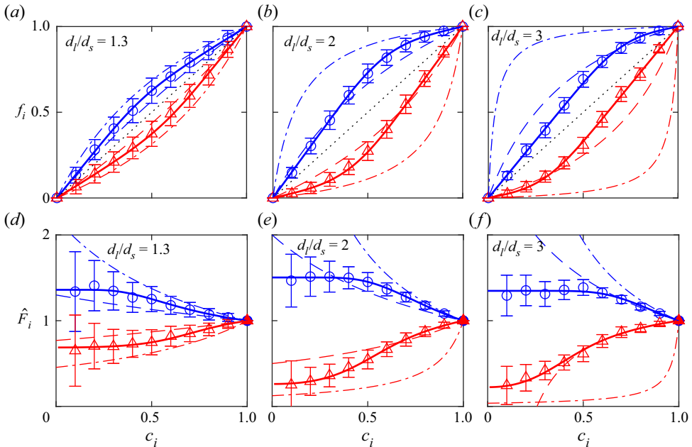
Figure 7. (a–c) Ratio of species-specific pressure to bulk pressure, f_i = P_i/P , for different size ratios. Symbols represent data for large ( \circ , blue) and small ( \triangle , red) particles. Solid curves are predictions of (3.3) recast as a pressure ratio, i.e. f_i = c_i \hat{F}_i . Thin curves are f_i as assumed in previous studies: f_i = d_i c_i / \sum(d_i c_i) (dashed) (Marks et al. 2012) and f_i = d_i^3 c_i / \sum(d_i^3 c_i) (dash-dot) (Tunuguntla et al. 2014). Dotted lines represent the monodisperse case ( d_l/d_s = 1 ) where f_i = c_i . (d–f) The dependence of the scaled segregation force, \hat{F}_i = f_i/c_i , on c_i for various models compared with simulation data and (3.3). Data and (3.3) fits are reproduced from figure 2(a–c).
