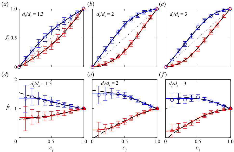
Figure 4. (a–c) Ratio of species-specific pressure to bulk pressure, f_i = P_i/P , for different size ratios. Symbols represent data for large ( \circ , blue) and small ( \triangle , red) particles. Solid curves are predictions of (3.3) recast as a pressure ratio, i.e. f_i = c_i \hat{F}_i . Dashed black curves are best fits of the quadratic (Gajjar & Gray 2014) model to the data for each size ratio, d_l/d_s . Dotted lines represent the monodisperse case ( d_l/d_s = 1 ) where f_i = c_i . (d–f) Scaled segregation force from simulation data (symbols), \hat{F}_i = f_i/c_i , is well fit over the full c_i range by (3.3) (solid curves) but poorly fit by the quadratic model (black dashed curves) at low c_i . Data and (3.3) fits are reproduced from figure 2(a–c).
