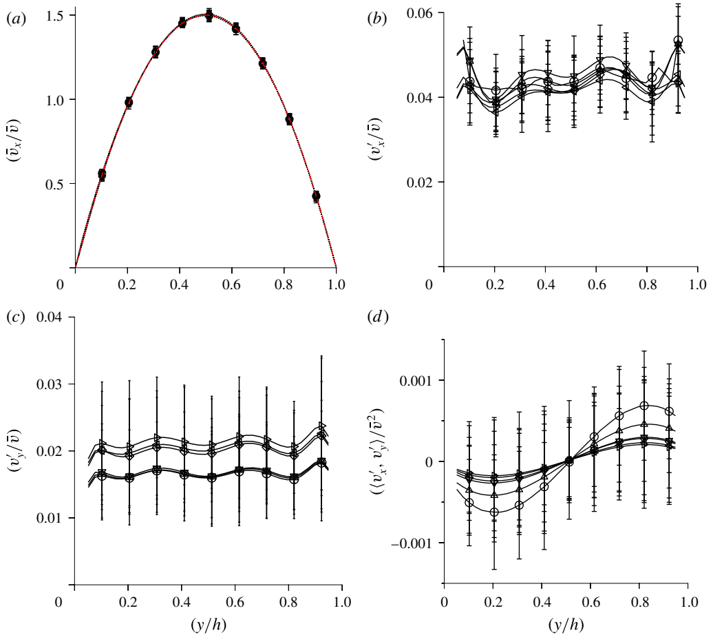
FIGURE 20. (Colour online) The cross-stream variation of \langle \bar{v}_x \rangle / \bar{v} (a), \langle v'_x v'_x \rangle / \bar{v} (b), \langle v'_y v'_y \rangle / \bar{v} (c) and \langle (v'_x v'_y) \rangle / \bar{v}^2 (d), at the streamwise location 0.5 cm upstream of the junction between the development and test sections at Reynolds number 217 ( \circ ), 403 ( \triangle ), 482 ( \nabla ), 597 ( \triangleleft ), 662 ( \triangleright ) and 814 ( \diamond ) for a channel with height approximately 0.6 mm in the undeformed state, when the walls are made with shear modulus 0.75 kPa. The dashed curve in panel (a) shows a parabolic velocity profile with the same mean velocity.
