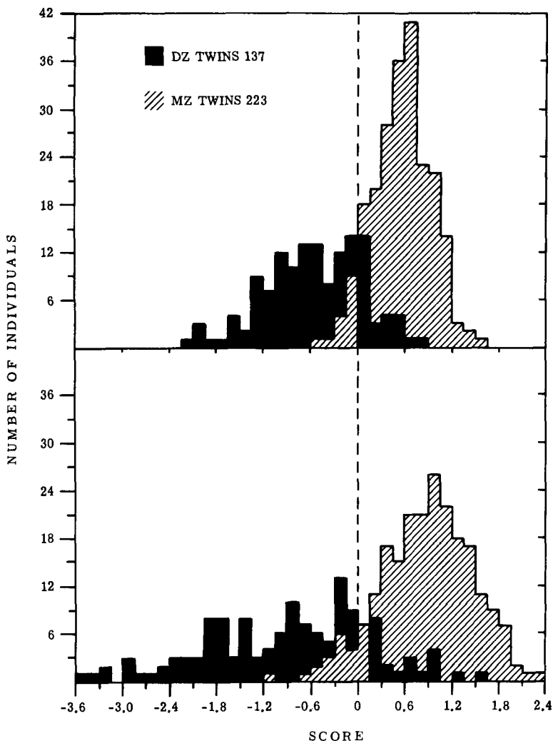
Figure. Distribution of discriminant scores using |A-B| and \left| \frac{(A+B)}{2} - \bar{x} \right| (top) compared with |A-B| alone (bottom). The overlap between MZ and DZ twins is less in the top histogram despite similar discrimination at a central cutoff point (dotted line).
