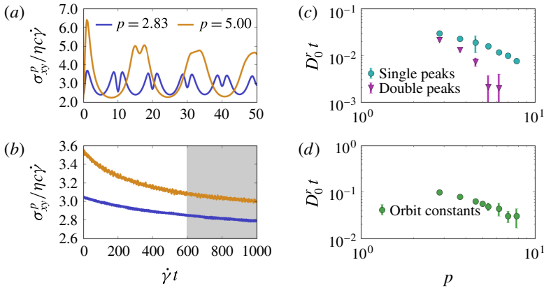
FIGURE 11. (Colour online) Rheology of a suspension of rod-like particles with orientations allowed to rotate freely in three dimensions, for particle aspect ratios p = 2.83 and p = 5.00 and Pe = 10^4 , drawn from two separate initial distributions: (a) equilibrated orbit constant but a single phase angle, and (b) equilibrated phase angle but single orbit constant. Note the difference in scale for both axes. (c) The decay times of the single- and double-peak structures in the suspension stress, from simulations over a range of aspect ratios. Since the double-peak structure decays extremely rapidly, our simulation cannot resolve the double-peak decay time for the last two aspect ratios p \approx 7 and p \approx 8 . (d) The decay time of the suspension stress at intermediate times due to the orbit constant relaxation, as a fit over the shaded time window in (b).
