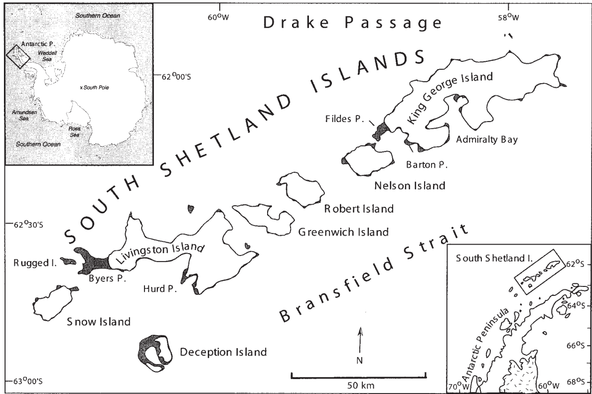
Fig. 1. Index map of the South Shetland Islands.
