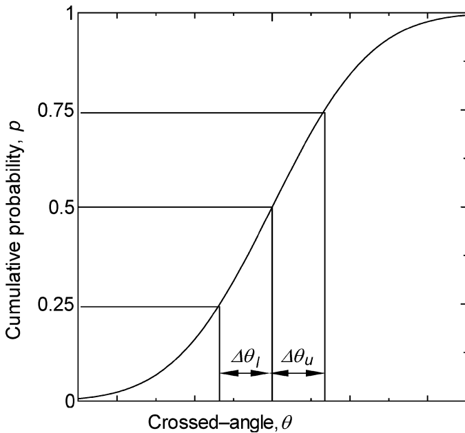
Fig. 10. Estimation method for upper and lower thresholds.
