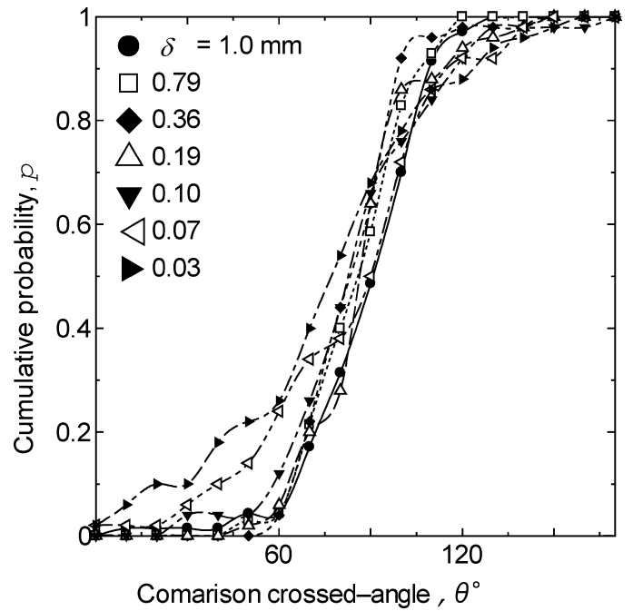
Fig. 16. Ogive curves obtained from experiments performed to evaluate presentable fringe height of virtual texture.
