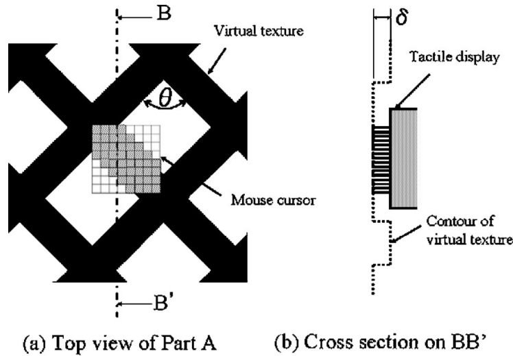
Fig. 9. Crossed-axis angle on the display area. (a) Top view. (b) Cross section (side view).
