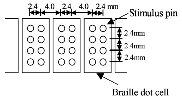
Fig. 2. Array of Braille dot cells.
