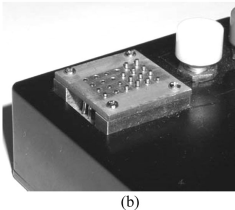
Fig. 4. Example of virtual figure presentation. (a) Virtual triangle and the cursor of a mouse. (b) Extruded stimulus pins on the tactile display panel according to the mouse cursor traveling on the virtual figure.
