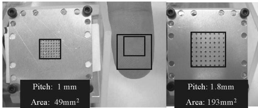
Fig. 5. Tactile display pads for display B; (left) 1-mm type; (middle) a finger for comparison; (right) 1.8-mm type.
