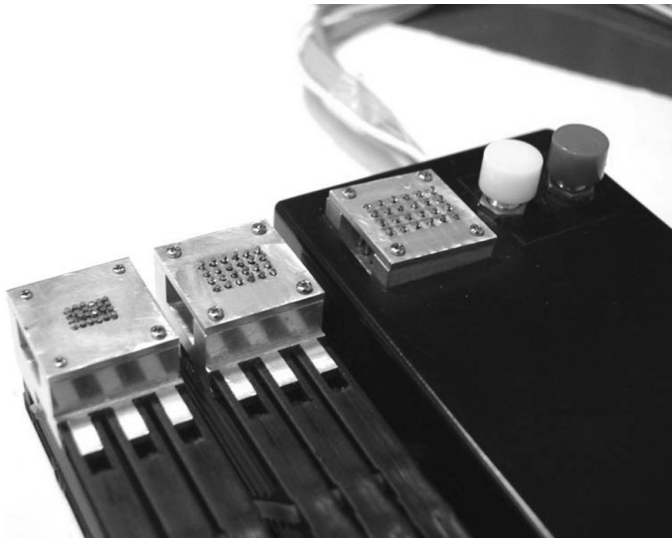
Fig. 3. Three tactile presentation pads for display A.
