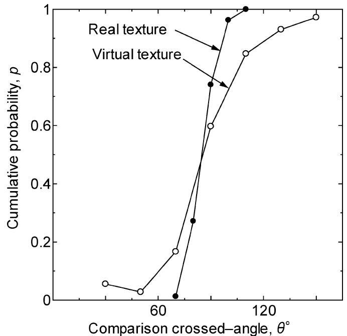
Fig. 19. Comparison of detection precision between virtual texture and real texture.
