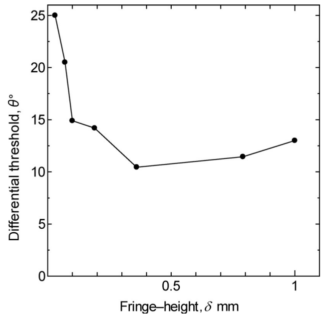
Fig. 17. Relationship between differential threshold and fringe height.
