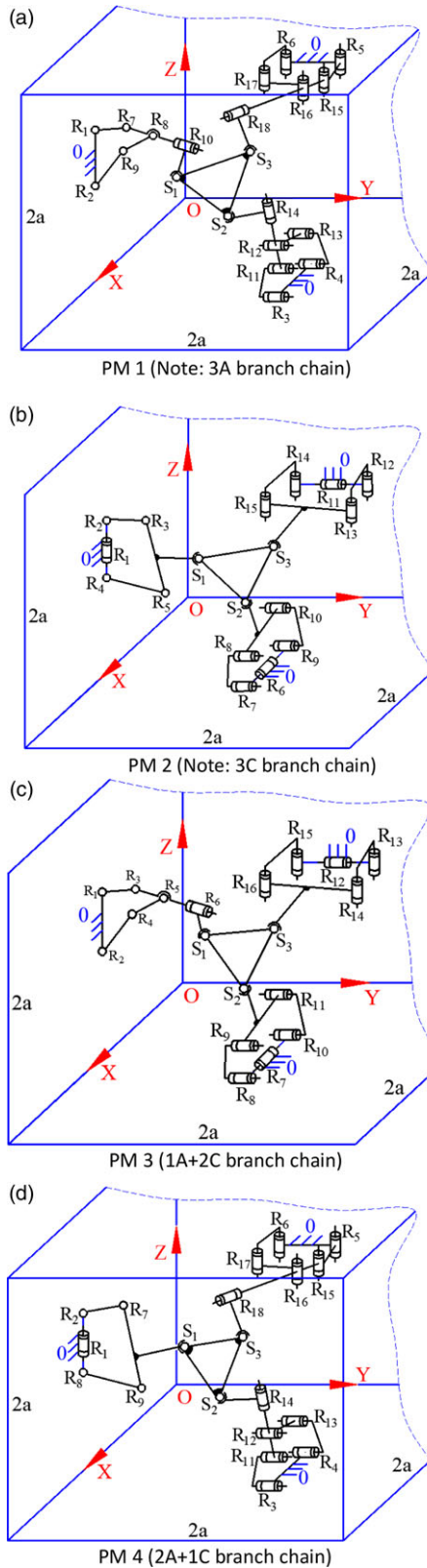
Figure 2. A class of four 6-DOF parallel mechanisms.
