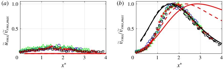
FIGURE 17. Root mean square data for \eta = 0 of the periodic part of the signal as a function of x^* : v_0 = 2.2 \times 10^{-5} . With (a) \tilde{u}_{rms}/\tilde{v}_{rms,max} , (b) \tilde{v}_{rms}/\tilde{v}_{rms,max} . Data points are for different frequencies: (○) 50 Hz, (△) 60 Hz, (*) 70 Hz, (□) 80 Hz. Theoretical stability analysis is shown with: ---- parallel theory, — weakly divergent theory (black lines with eddy-viscosity model, red lines without eddy-viscosity model). Note that the stability analysis gives \tilde{u}_{rms} = 0 on the centreline since only sinuous modes are considered.
