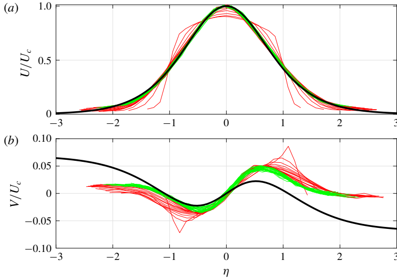
FIGURE 4. Profiles of the mean streamwise (a) and transverse (b) velocities. Profiles for x < 15 are coloured in red, whereas those for x > 15 are coloured in green. Black lines show the theoretical profiles.
