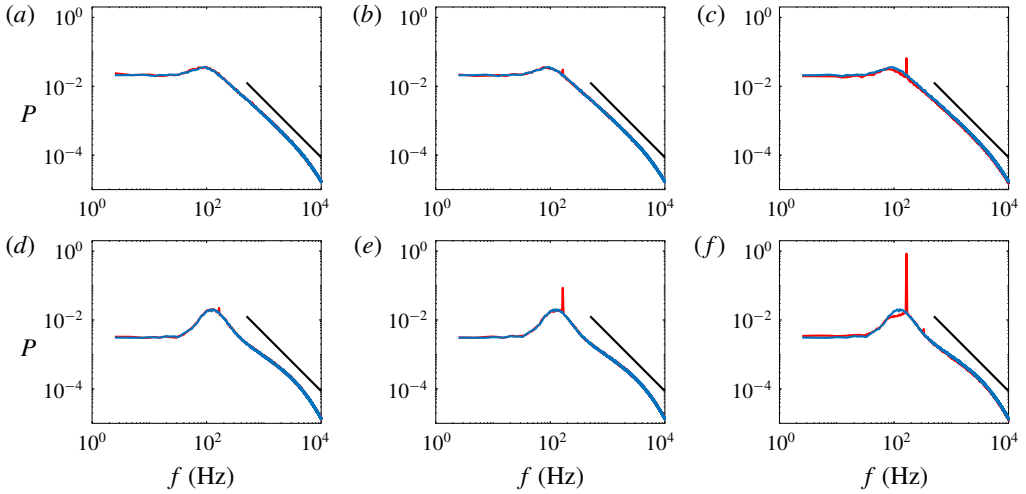
FIGURE 9. Power spectra distributions for the streamwise (a–c) and transverse velocity component (d–f) for three excitation amplitudes: (a, d) v_0 = 3.9 \times 10^{-5} , (b, e) v_0 = 1.2 \times 10^{-4} and (c, f) v_0 = 3.9 \times 10^{-4} all in red, while the blue lines indicate the unexcited spectra. The spectra are evaluated at x = 16 , y = 0.117 ( \eta = 0.07 ), f = 165 Hz. Black lines show the power law f^{-5/3} .
