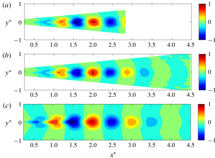
FIGURE 16. Contour maps of \tilde{v} at v_0 = 2.2 \times 10^{-5} : (a) f = 50 Hz, (b) f = 100 Hz, (c) weakly divergent linear theory. The fields are scaled by the transverse velocity perturbation at x^* = 2 .
