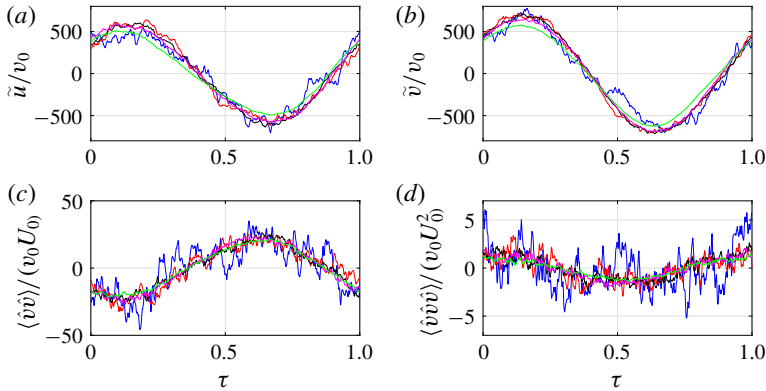
FIGURE 10. Signals of (a) \langle u \rangle / v_0 = \tilde{u} / v_0 , (b) \langle v \rangle / v_0 = \tilde{v} / v_0 , (c) \langle \tilde{v}^2 \rangle / (v_0 U_0) and (d) \langle \tilde{v}^3 \rangle / (v_0 U_0^2) at x = 19.5 and \eta = 1 for f = 50 Hz and five different excitation amplitudes. With (blue) v_0 = 6.9 \times 10^{-6} , (red) v_0 = 1.2 \times 10^{-5} , (black) v_0 = 2.2 \times 10^{-5} , (magenta) v_0 = 3.9 \times 10^{-5} , (green) v_0 = 6.9 \times 10^{-5} .
