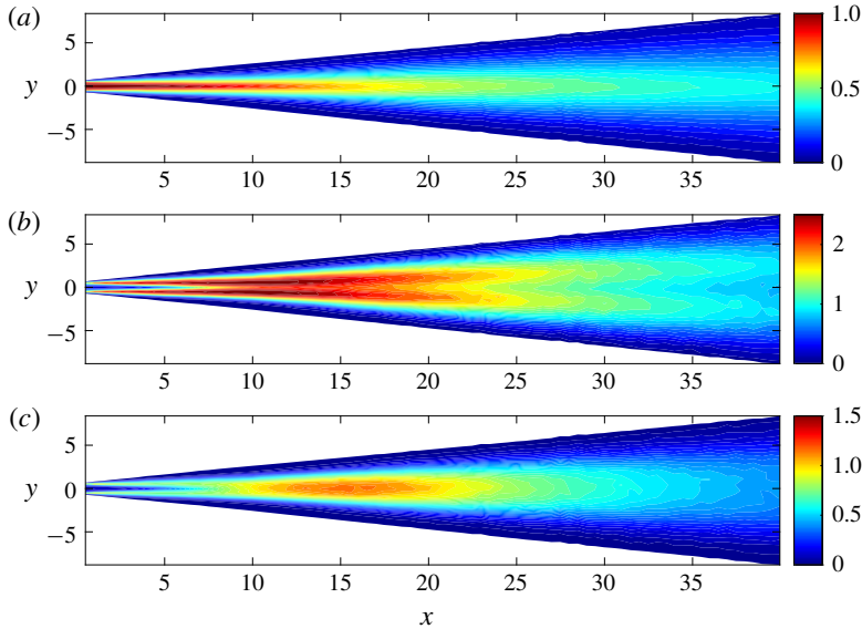
FIGURE 2. Contour maps of (a) U , (b) 100\overline{uu} and (c) 100\overline{vv} for the unexcited jet.
