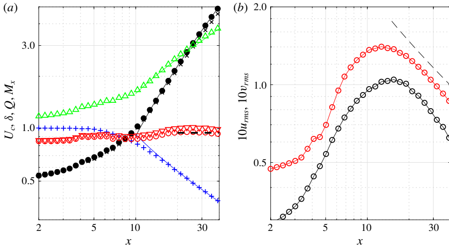
FIGURE 3. (a) Streamwise evolution of integral jet properties without initial forcing. With (black circles) \delta from the fitting, (black crosses) \delta from the direct integration, (blue pluses) measured U_c , (green triangles) mass flux, Q , (red circles) momentum flux, M_x , (red triangles) mean and turbulent momentum flux, M_x + m_x . The lines are obtained by fitting the experimental data in the last 20d demonstrating that U_c \propto 1/\sqrt{x - x_0} , \delta \propto x - x_0 and M_x = 4/3U_c^2\delta = \text{const.} , according to the theory described in § 3. (b) Streamwise distributions of 10u_{rms} (red circles), 10v_{rms} (black circles) along the jet centreline, (dashed line) u_{rms} \propto 1/\sqrt{x - x_0} . Both plots have been interpolated to a logarithmic grid to enhance the visibility of the theoretical trends.
