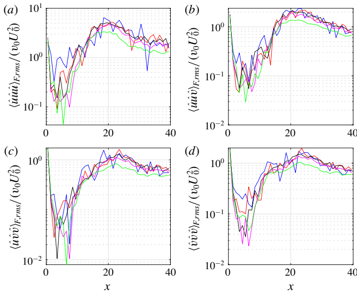
FIGURE 12. Streamwise distributions of the r.m.s. of the filtered phase-averaged third-order correlations at \eta = 1 and f = 50 Hz. The colour scheme is the same as the one used in figure 10.
