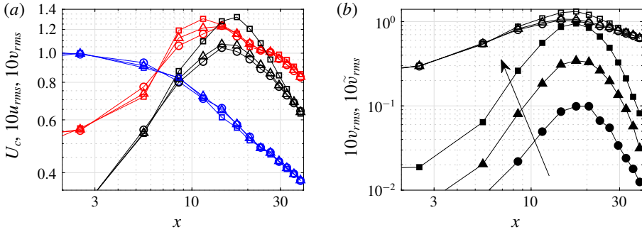
FIGURE 6. (a) Streamwise distributions of U_c (blue), 10u_{rms} (red), 10v_{rms} (black) along the jet centreline for three different initial forcing amplitudes with f = 100 Hz. (b) v_{rms} (open symbols) and \tilde{v}_{rms} (filled symbols). The three different initial forcing amplitudes are denoted by: \circ v_0 = 2.2 \times 10^{-5} , \triangle v_0 = 6.9 \times 10^{-5} , \square v_0 = 2.2 \times 10^{-4} . The arrow in (b) indicates the increasing forcing amplitude, as a visual aid. Not all data points are shown since it would lead to overcrowding of the figure.
