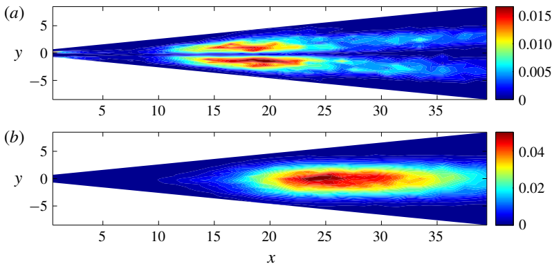
FIGURE 7. Contour maps of (a) 100\tilde{u}_{rms}^2 and (b) 100\tilde{v}_{rms}^2 for the excited jet at f = 50 Hz.
