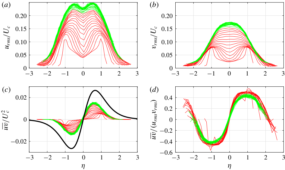
FIGURE 5. Distributions of the velocity fluctuations. Colouring of the lines as in figure 4. (a) u_{rms}/U_c , (b) v_{rms}/U_c , (c) \overline{u\overline{v}}/U_c^2 , (d) \overline{u\overline{v}}/(u_{rms}v_{rms}) . The black line in (c) shows equation (3.20).
