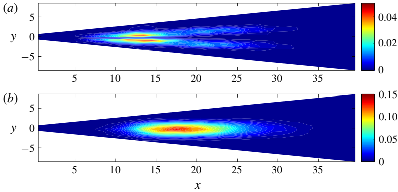
FIGURE 8. Contour maps of (a) 100\tilde{u}_{rms}^2 and (b) 100\tilde{v}_{rms}^2 for the excited jet at f = 100 Hz.
