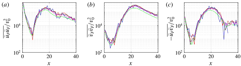
FIGURE 14. Distributions of filtered (a) \overline{\tilde{u}_F \tilde{u}_F} / v_0^2 , (b) \overline{\tilde{v}_F \tilde{v}_F} / v_0^2 , (c) \overline{\tilde{u}_F \tilde{v}_F} / v_0^2 at \eta = 1 . Same conditions as in figure 10.
