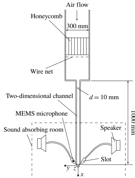
FIGURE 1. Experimental set-up of the two-dimensional turbulent jet.
