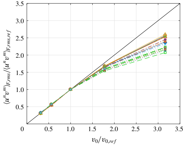
FIGURE 13. Proportionality of \langle u \rangle , \langle v \rangle and \langle \hat{u}^n \hat{v}^m \rangle against v_0 . All moments are evaluated at \eta = 1 and averaged in 14.5 \leq x \leq 34.5 ; 2 \leq n + m \leq 5 ; v_{0,ref} = 2.2 \times 10^{-5} .
