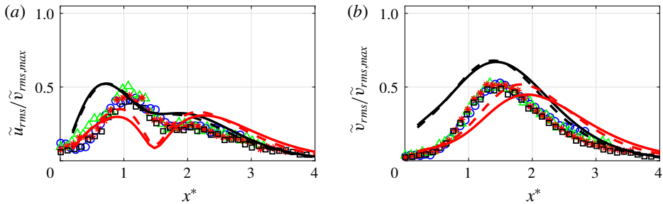
FIGURE 18. Root mean square data for \eta = 1 of the periodic part of the signal as a function of x^* : v_0 = 2.2 \times 10^{-5} . With (a) \tilde{u}_{rms}/\tilde{v}_{rms,max} , (b) \tilde{v}_{rms}/\tilde{v}_{rms,max} . Data points are for different frequencies: (○) 50 Hz, (△) 60 Hz, (*) 70 Hz, (□) 80 Hz. Theoretical stability analysis is shown with: ---- parallel theory, — weakly divergent theory (black lines with eddy-viscosity model, red lines without eddy-viscosity model).
