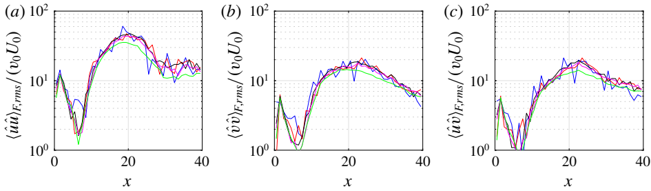
FIGURE 11. Distributions of (a) \langle \hat{u}\hat{u} \rangle_{F,rms} / (v_0 U_0) , (b) \langle \hat{v}\hat{v} \rangle_{F,rms} / (v_0 U_0) , (c) \langle \hat{u}\hat{v} \rangle_{F,rms} / (v_0 U_0) at \eta = 1 filtered around the forcing frequency ( f = 50 Hz). The colour scheme is the same as the one used in figure 10.
