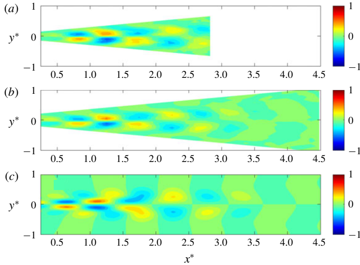
FIGURE 15. Contour maps of \tilde{u} at v_0 = 2.2 \times 10^{-5} : (a) f = 50 Hz, (b) f = 100 Hz, (c) weakly divergent linear theory. The fields are scaled by the transverse velocity perturbation at x^* = 2 .
