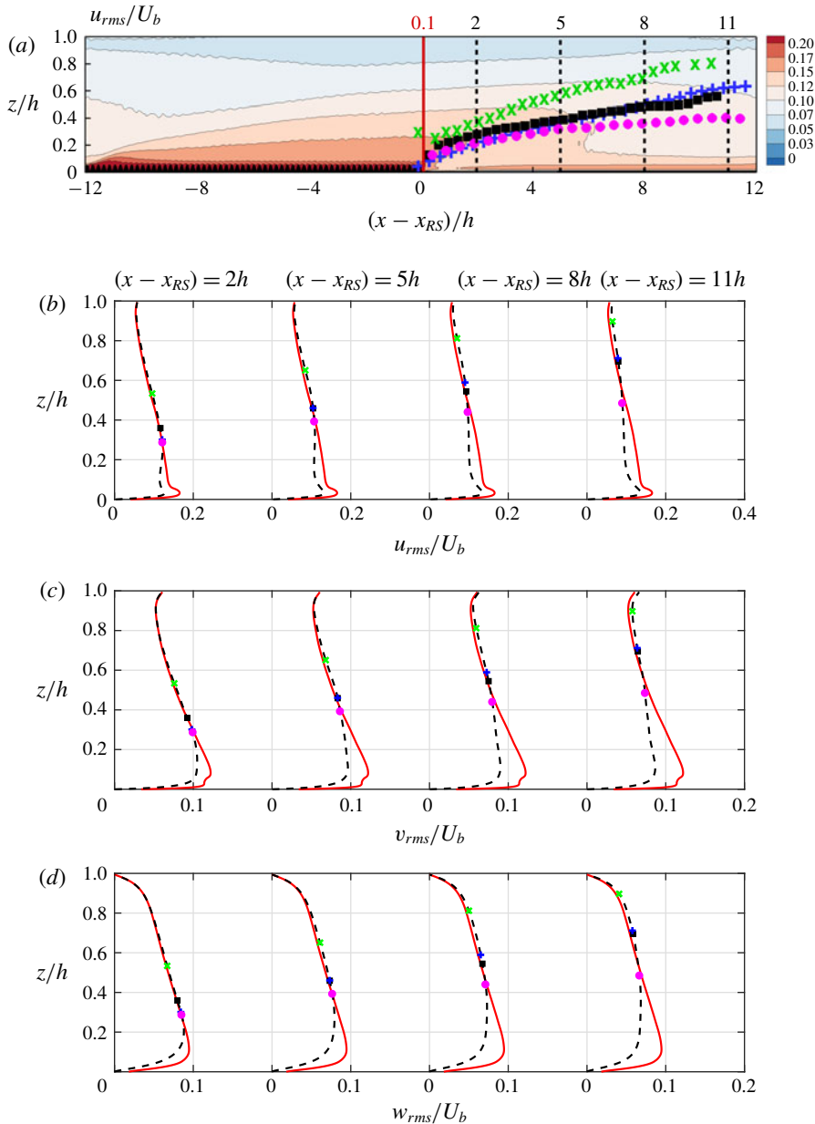
FIGURE 22. (Colour online) (a) The u_{rms} field overlaid with the IBL definitions. Comparison of profiles of (b) u_{rms} , (c) v_{rms} and (d) w_{rms} , after a fetch of 2h , 5h , 8h and 11h over the smooth patch (---), with their upstream counterparts after a fetch of 0.1h (—). The extracted locations are indicated in the u_{rms} field in (a). The four overlaid IBL definitions are: \delta_{AW} (■), \delta_{BMP} (+), \delta_{SP} (×) and \delta_E (●). The spanwise projection of the ‘egg-carton’ roughness is indicated with black colour.
