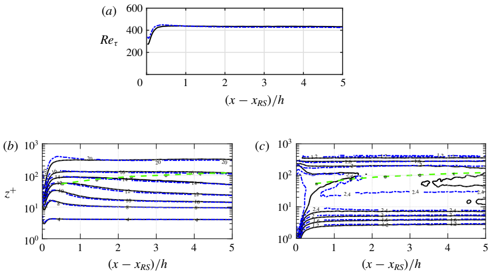
FIGURE 25. (Colour online) Comparison of statistics between case 12h (-----) and non-periodic case (—) during rough-to-smooth step change. (a) Reynolds number Re_\tau ; and contour lines of (b) U^+ and (c) u_{rms}^+ . Quantities in plus units are normalised by the local u_\tau and \nu . The IBL thickness, defined by Elliott (1958), is overlaid on the contour lines (—○—).
