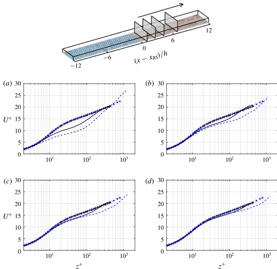
FIGURE 12. (Colour online) Rough-to-smooth comparison of U^+ profiles between case 24h (—) and DNS of Ismail et al. (2018) (---). Comparison is made at the several (x - x_{RS}) locations (shown in the domain): (a) 0.8h ; (b) 2.5h ; (c) 4.1h ; (d) 7.5h . Fully recovered flow for case 24h at Re_\tau = 437 (+) and Ismail et al. (2018) at Re_\tau = 1115 (×).
