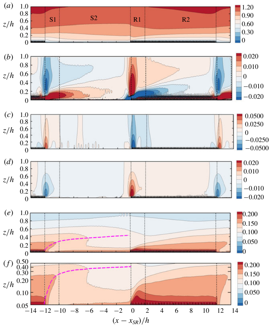
FIGURE 7. Variations of (a) U/U_b , (b) (h/U_b)(\partial U/\partial x) , (c) [h/(\rho U_b^2)](\partial P/\partial x) , (d) W/U_b and (e,f) u_{rms}/U_b , scaled by the bulk velocity U_b and h . The regions over the smooth patch (S1 + S2) and rough patch (R1 + R2) are separated into zones S1 and R1 that cover a fetch of 2h , and zones S2 and R2 that cover the remaining portions. The fields are overlaid by the spanwise projection of the roughness, in black colour. In (c) the total pressure gradient \partial P/\partial x includes the driving -\rho G and periodic \partial \tilde{P}/\partial x parts. In (f) the z -axis is in log scale to highlight the near-wall region. The outer peak of u_{rms} over the smooth patch is marked with (---).
