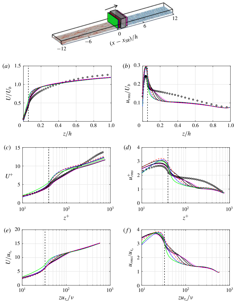
FIGURE 13. (Colour online) Profiles of (a,c,e) U and (b,d,f) u_{rms} up to a fetch of 2h over the rough patch, zone R1. Normalisation is consistent with figure 8. The vertical dashed line locates the roughness crest. The black curves are equally spaced in the range 0.8h \leq (x - x_{SR}) \leq 1.8h , (x - x_{SR}) = 0.2h (—), 0.4h (---), blue), 0.6h (---), magenta). Fully developed open channel over homogeneous ‘egg-carton’ roughness (○), with k/h = 0.056 at Re_{\tau} = 704 .
