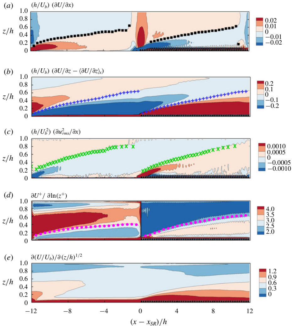
FIGURE 16. (Colour online) Application of the definitions of \delta_i in table 5 to case 24h. (a) AW, (b) BMP, (c) SP, (d) E, (e) AL. In each panel the contour plot shows the characteristic parameter to identify \delta_i , and the symbols locate \delta_i based on the corresponding definition ( \delta_{AW} (■), \delta_{BMP} (+), \delta_{SP} (×), \delta_E (●)). In (e) detecting \delta_i from AL was not straightforward (refer to text). The fields are overlaid by the spanwise projection of the roughness, in black colour.
