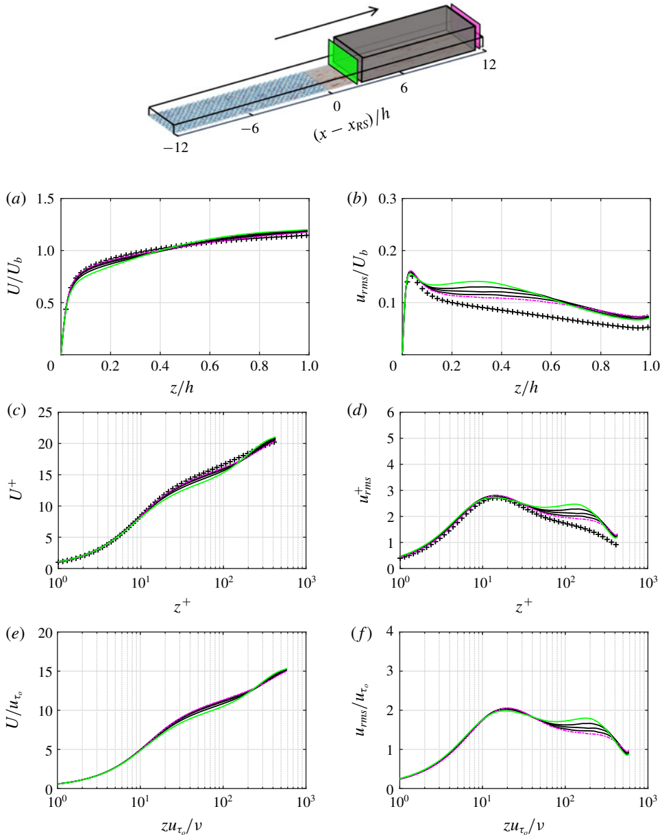
FIGURE 11. (Colour online) Profiles of (a,c,e) U and (b,d,f) u_{rms} for 3h \leq (x-x_{RS}) \leq 11h , zone S2. Normalisation is consistent with figure 8. The black curves are equally spaced in the range 5h \leq (x-x_{RS}) \leq 9h (the shadowed box). Here (x-x_{RS})=3h (—) and 11h (----). DNS of fully developed smooth open-channel flow at Re_{\tau}=437 (+).
