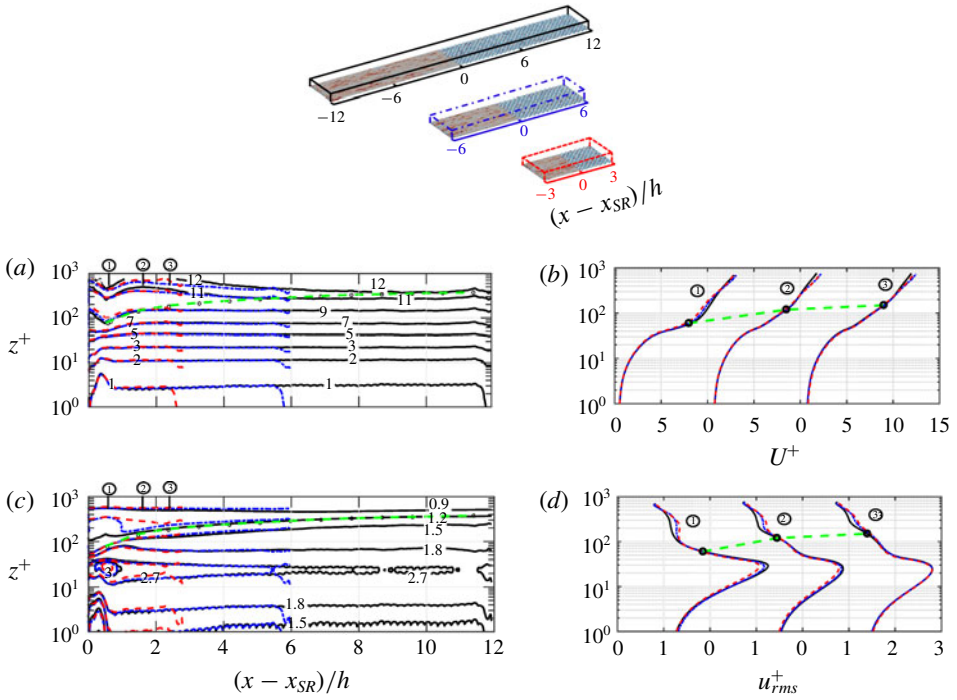
FIGURE 5. (Colour online) Contour lines of (a) U^+ and (c) u_{rms}^+ for the three domain lengths over the rough patch. The x -origin is placed at x_{SR} (consider the top domains). Profiles of (b) U^+ and (d) u_{rms}^+ at several (x - x_{SR})/h : ① 0.5h , ② 1.5h and ③ 2.5h . Legends are consistent with those of figure 3. Quantities in plus units are normalised by the local u_\tau and \nu . The IBL thickness, defined by Elliott (1958), is overlaid on the contour lines and profiles (---○---).
