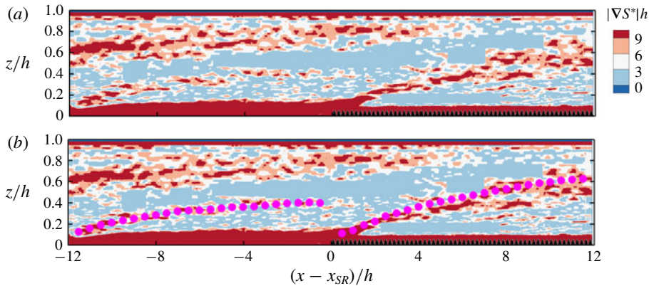
FIGURE 21. (Colour online) The gradient magnitude of S^* ( |\nabla S^*| ) corresponding to figure 20 is shown in (a) and (b). In (b) |\nabla S^*| is overlaid with \delta_E (●). The fields are overlaid by the spanwise projection of the roughness, in black colour.
