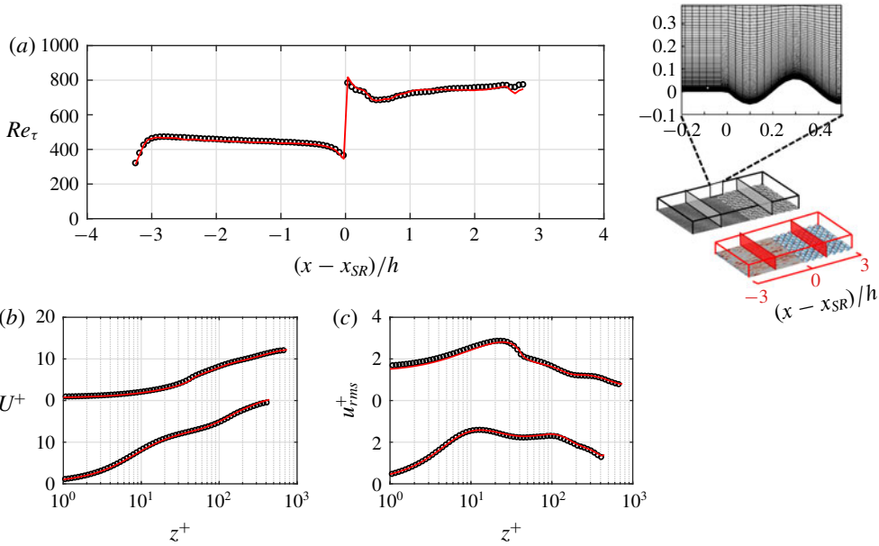
FIGURE 23. (Colour online) Comparison between cases 6h (—) and 6h verification (○). (a) Reynolds number Re_\tau based on local u_\tau and h . Profiles of (b) U and (c) u_{rms} . The quantities in plus units are normalised by the local u_\tau and v . Comparison is made in the middle of the smooth patch (lower curves in b,c) and in the middle of the rough patch (upper curves in b,c), demonstrated in the domains on the right-hand side.
