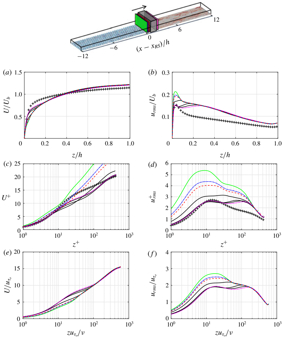
FIGURE 8. (Colour online) Profiles of (a,c,e) U and (b,d,f) u_{rms} up to a fetch of 2h over the smooth patch, zone S1. Profiles are normalised by (a,b) U_b, h , (c,d) local u_\tau and v and (e,f) u_{\tau_o} and v . The black curves are equally spaced in the range 0.2h \leq (x - x_{RS}) \leq 1.8h (the shadowed box at the top). Here (x - x_{RS}) = 0.05h (—), 0.08h (-----, blue), 0.1h (---) and 2h (-----, magenta); DNS of fully developed smooth open-channel flow at Re_\tau = 437 (+).
