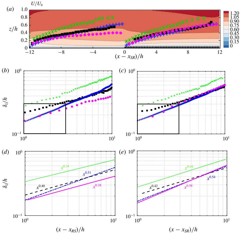
FIGURE 19. (Colour online) Comparison between the definitions of \delta_i throughout the domain in linear scale (a). The resulting \delta_i plotted in log scale over (b) the smooth patch and (c) the rough patch. Note that the origin has been shifted to the beginning of the smooth patch ( x_{RS} ) in (b,d). Power-law fitting the resulting \delta_i over (d) the smooth patch and (e) the rough patch. Definitions: \delta_{AW} (■, ---); \delta_{BMP} (+, - - - -); \delta_{SP} (×, - - - -); \delta_E (●, —). The framed regions in (b,c) highlight the close behaviour of \delta_E and \delta_{BMP} within a fetch of 3h .
