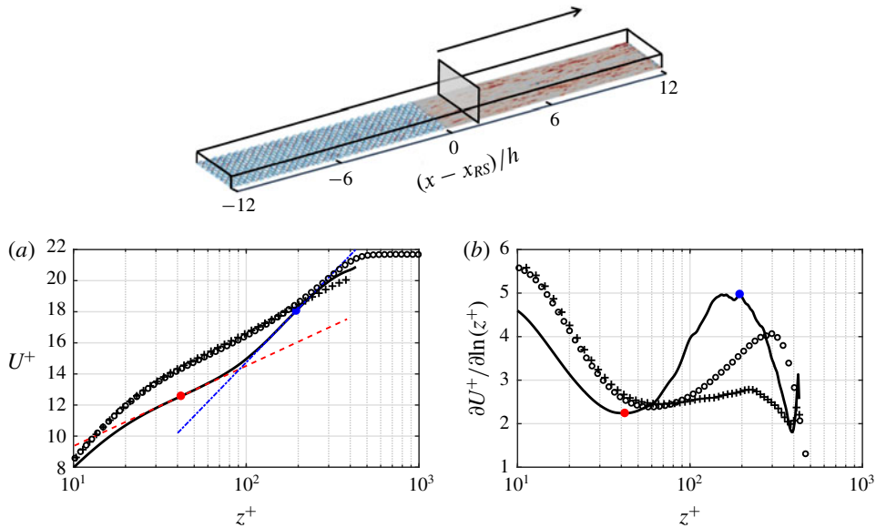
FIGURE 9. (Colour online) Profiles of (a) U^+ and (b) its logarithmic slope \partial U^+ / \partial \ln(z^+) for case 24h at (x - x_{RS}) = 2h (—), indicated in the top domain. The inner and outer logarithmic slopes are identified through the extrema of \partial U^+ / \partial \ln(z^+) (●, red; ●, blue). The fitting lines (---) and (- - - -) have the same slopes as the extrema. Fully developed open-channel flow at Re_\tau = 437 (+). Canonical boundary layer at Re_\tau \simeq 445 (○) by Jiménez et al. (2010).
