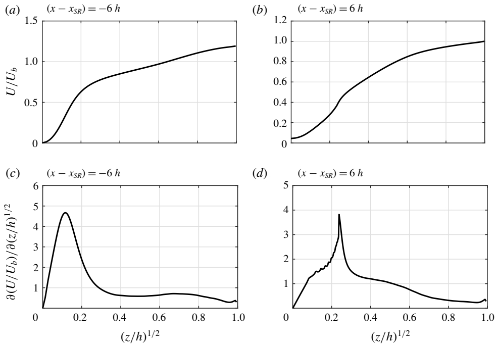
FIGURE 18. Profiles of (a,b) U/U_b versus (z/h)^{1/2} at the same locations indicated in figure 17. Profiles of (c,d) the slope curves, \partial(U/U_b)/\partial(z/h)^{1/2} , corresponding to the profiles in (a,b).
