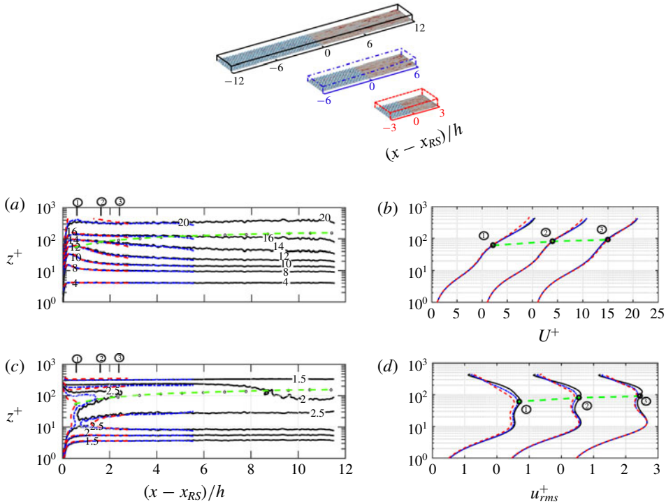
FIGURE 4. (Colour online) Contour lines of (a) U^+ and (c) u_{rms}^+ for the three domain lengths over the smooth patch. The x -origin is placed at x_{RS} (consider the top domains). Profiles of (b) U^+ and (d) u_{rms}^+ at several (x - x_{RS})/h : ① 0.5h , ② 1.5h and ③ 2.5h . Legends are consistent with those of figure 3. Quantities in plus units are scaled by the local u_\tau and v . The IBL thickness, defined by Elliott (1958), is overlaid on the contour lines and profiles (—○—).
