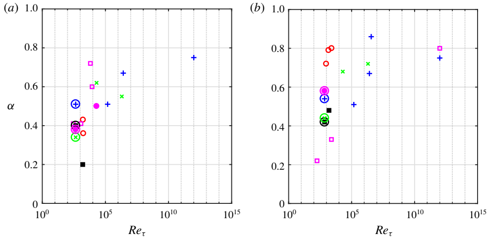
FIGURE 15. (Colour online) Values of the power-law exponent \alpha for \delta_i from the previous studies in table 5. Studies that have adopted the same definition of \delta_i are indicated with the same symbol. (a) Rough-to-smooth and (b) smooth-to-rough step change. AW (■); AL (○); BMP (+); SP (×); E (●); PA (□). The circled symbols at Re_\tau = 443 (a) and Re_\tau = 715 (b) are obtained from application of different definitions of \delta_i to case 24h.
