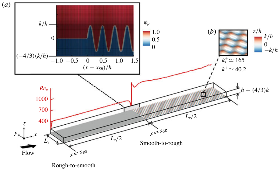
FIGURE 2. (Colour online) Computational domain equally divided between the smooth and rough patches. The bottom solid surface is identified with iso-surface of \phi_p = 0.5 . Here \phi_p is the volume of fluid for the pressure cells (appendix A). (a) Side view of the domain, at the smooth-to-rough surface change overlaid by the grid. (b) The roughness elements, coloured by z/h . The red curve is the friction Reynolds number Re_\tau \equiv u_\tau h/\nu based on the local u_\tau .
