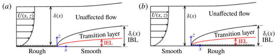
FIGURE 1. (Colour online) Schematic representation of the IBL, IEL and transition layer, adopted from Savelyev & Taylor (2005), for a boundary layer over (a) a rough-to-smooth step change and (b) a smooth-to-rough step change. Here U(x, z) denotes the streamwise velocity, averaged over time and spanwise direction, and \delta(x) and \delta_i(x) are the boundary layer and IBL thicknesses, respectively.
