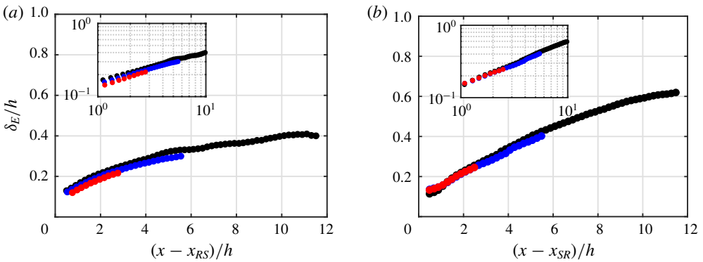
FIGURE 6. (Colour online) IBL thickness defined by Elliott (1958) ( \delta_E , discussed in § 3.3) over (a) the smooth patch and (b) the rough patch. Cases 6h (●, red), 12h (●, blue) and 24h (●, black). The insets are the same plots using log–log scales.
