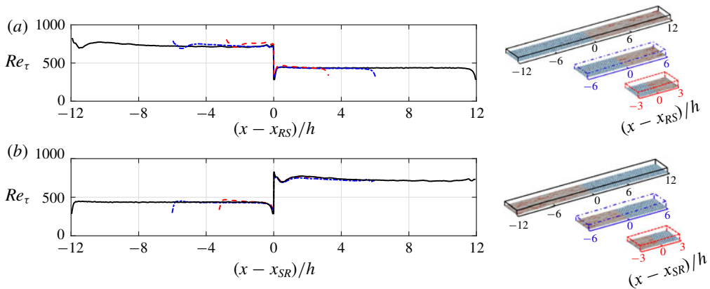
FIGURE 3. (Colour online) Comparison of the local Re_\tau between cases 6h (---), 12h (-·-·-) and 24h (—), the cases being shown on the right. Comparison over (a) the smooth patch and (b) the rough patch. The x -origin is placed at (a) x_{RS} and (b) x_{SR} .
