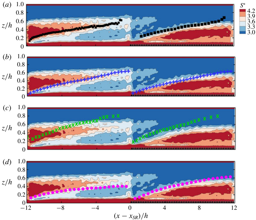
FIGURE 20. (Colour online) The normalised mean shear rate S^* = |S|\mathcal{K}/\varepsilon , overlaid with the IBL definitions: (a) \delta_{AW} (■), (b) \delta_{BMP} (+), (c) \delta_{SP} (×) and (d) \delta_E (●). The fields are overlaid by the spanwise projection of the roughness, in black colour.
