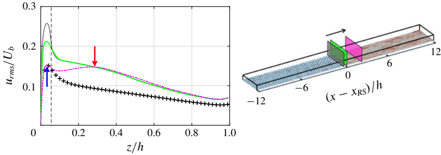
FIGURE 10. (Colour online) Profiles of u_{rms} , normalised by U_b , at (x - x_{RS}) = -0.05h (---), 0.05h (—) and 2h (----), indicated in the domain on the right. The vertical dashed line locates the roughness crest ( z = k ). The upward and downward arrows indicate the inner and outer peaks of (----).
