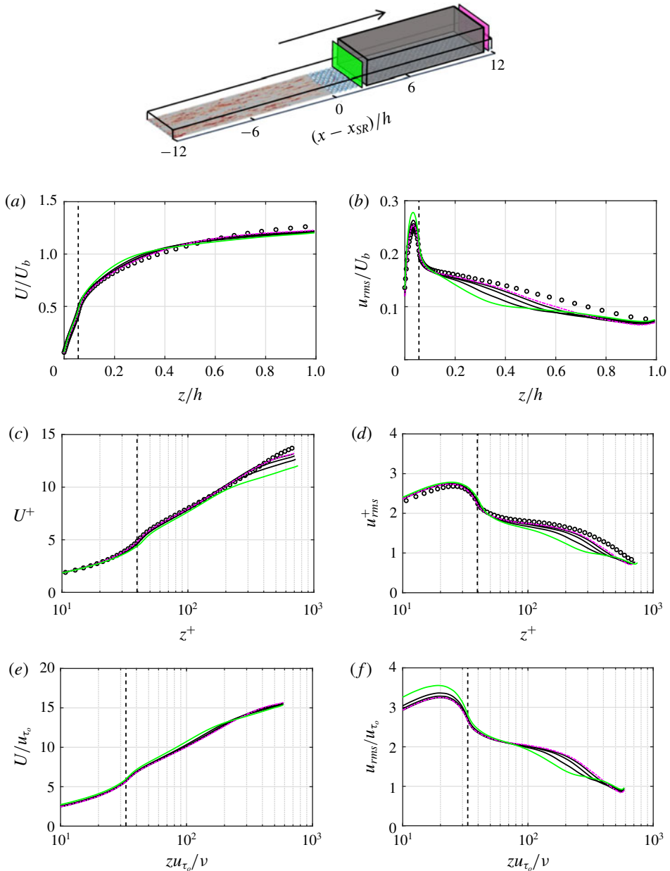
FIGURE 14. (Colour online) Profiles of (a,c,e) U and (b,d,f) u_{rms} for 3h \leq (x - x_{SR}) \leq 11h , zone R2. Normalisation is consistent with figure 8. The black curves are equally spaced in the range 5h \leq (x - x_{SR}) \leq 10h , (x - x_{SR}) = 3h (—) and 11h (----). Fully developed open channel over homogeneous ‘egg-carton’ roughness (O), with k/h = 0.056 at Re_\tau = 704 .
