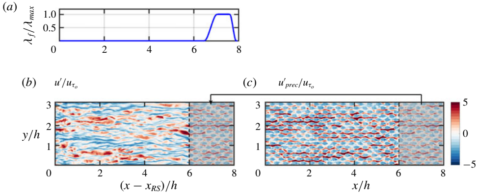
FIGURE 24. (Colour online) Illustration of concurrent precursor method (Stevens et al. 2014; Munters et al. 2016) for the rough-to-smooth non-periodic set-up with fully recovered inflow. (b) The main domain and (c) the precursor domain at z u_{\tau_0}/\nu = 15 . The shaded regions indicate the data extraction region in (c) and the fringe forcing region in (b). (a) The fringe masking function \lambda_f normalised by \lambda_{max} = 3000 .
