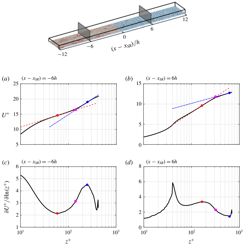
FIGURE 17. (Colour online) Identifying \delta_E from logarithmic slope change. The quantities are normalised by the local u_\tau and v . Profiles of (a,b) U^+ at (x - x_{SR}) = -6h and 6h , indicated in the computational domain. Profiles of (c,d) \partial U^+ / \partial \ln(z^+) corresponding to the profiles in (a,b). The inner and outer slopes are the extrema of \partial U^+ / \partial \ln(z^+) (●, red; ●, blue). Here \delta_E (●, magenta) is located by intersecting the inner (---) and outer (-----) logarithmic fitting lines.
