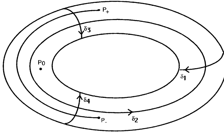
FIGURE 3. The vanishing cycles on the elliptic curve \Gamma_h, -\frac{1}{2} < a < 0 .
