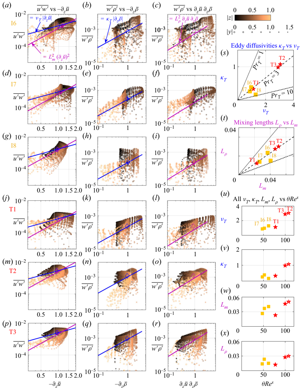
Figure 10. Eddy diffusivities and mixing lengths in data sets I6–T3 (top to bottom row). Clouds of n_y n_z points of \overline{u'w'} \equiv \mathcal{P}/\overline{S} vs -\partial_z \overline{u} \equiv \overline{S} (first column); \overline{w'\rho'} \equiv \mathcal{B}/Ri_b^s vs -\partial_z \overline{\rho} \equiv \overline{N}^2/Ri_b^s (second column); \overline{w'\rho'} \equiv \mathcal{B}/Ri_b^s vs \partial_z \overline{u} \partial_z \overline{\rho} \equiv \overline{S}\overline{N}^2/Ri_b^s (third column). Note the log–log axes, and symbol colour and size respectively indicating the |z| and |y| location. Linear and quadratic least-squares fits provide the eddy diffusivities (in blue, after multiplying by Re^s as in (5.1a,b)) and mixing lengths (in purple). Diamonds show the volume-averaged values of the flux vs gradient (blue) or square gradient (purple). (s–x) The \nu_T, \kappa_T, L_m, L_\rho values (s–t) against one another, giving the ratio Pr_T = \kappa_T/\nu_T = L_\rho^2/L_m^2 ( Pr_T = 1, 3, 10 shown); (u–x) against the input parameters \theta Re^s . Values obtained from the fit are indistinguishable from those obtained from the diamonds.
