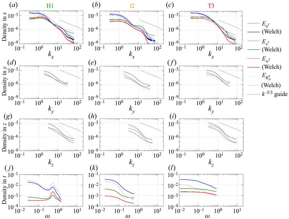
Figure 5. Spectral density of energy in individual velocity components u' (blue), v' (green), w' (red) and of K'_\rho (grey) in all directions x ( a-c ), y ( d-f ), z ( g-i ) and t ( j-l ) for three representative data sets H1 ( a,d,g,j ), I2 ( b,e,h,k ) and T3 ( c,f,i,l ). The mean energies (1/2)\langle u'^2 \rangle , (1/2)\langle v'^2 \rangle , (1/2)\langle w'^2 \rangle and \langle K'_\rho \rangle are given by one-dimensional integration of any respective density, e.g. (1/2)\langle u'^2 \rangle = \int_0^{k_x, \max} E_{u'}^x dk_x = \int_0^{k_y, \max} E_{u'}^y dk_y = \int_0^{k_z, \max} E_{u'}^z dk_z = \int_0^{\omega, \max} E_{u'}^t d\omega , etc. Mean values at k_x, k_y, k_z, \omega = 0 are not shown for clarity. The spectral range depends on domain length and resolution (k_x, k_y, k_z, \omega) \in [\pi/L_x, \pi/dx] \times [\pi/L_y, \pi/dy] \times [\pi, \pi/dz] \times [2\pi/L_t, \pi/dt] . Note the different axis scales between ( a-i ) and ( j-l ). In x , we compare spectra obtained by the standard DFT (thin lines) and by Welch's method (thick lines). In y, z we only show the former, and in t we only show the latter (see text for more details).
