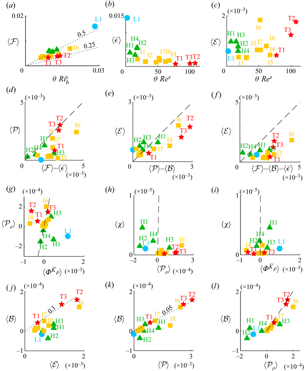
Figure 2. Steady-state energy fluxes in all 16 data sets. (a) Mean kinetic energy forcing (power source) as function of \theta Re_b^s . (b–c) Mean kinetic energy dissipation, and turbulent kinetic energy dissipation (power sinks) as function of \theta Re^s ( \approx \theta Re^h identified as proxy for regime transitions in LPL19). (d–f) Test of the approximate kinetic balances (2.7a), (2.8a), (2.8b), respectively. (g–i) Test of the approximate scalar variance balances (2.7c), (2.8c), (2.8d), respectively. (j–l) Test of three further commonly used ratios: \langle \mathcal{B} \rangle / \langle \mathcal{E} \rangle \equiv \Gamma , \langle \mathcal{B} \rangle / \langle \mathcal{P} \rangle \equiv R_f , and \langle \mathcal{B} \rangle / \langle \mathcal{P}_\rho \rangle ( \equiv 1 when \partial_z \bar{\rho} = 1 ), respectively. All dashed lines have slope 1 and denote expected equality between fluxes. Dotted lines are labelled explicitly.
