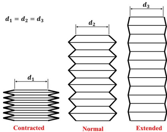
Figure 9. Example of creased bellows and their mechanism.
