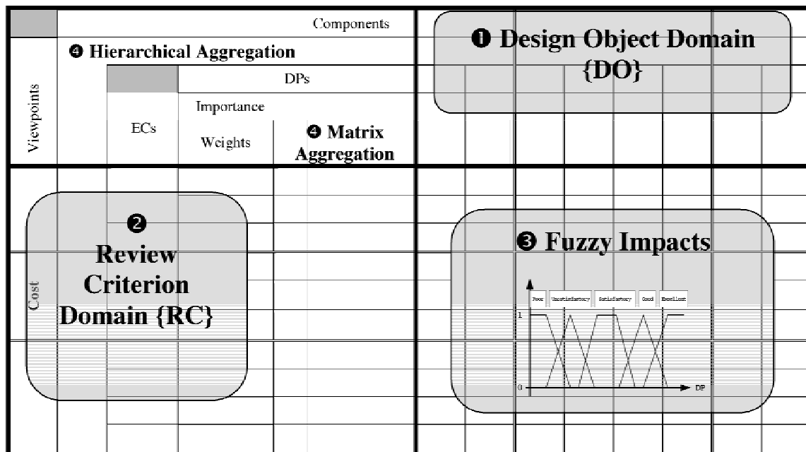
Fig. 1. An overview and the steps of FuzzySTAR.
