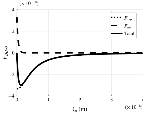
FIGURE 20. DLVO curve for A_H = 1 \times 10^{-20} J, D_p = 20 \mu\text{m} , \zeta_0 = R_p \times 5 \times 10^{-4} , and C_{\text{salt}} = 35 ppt.
