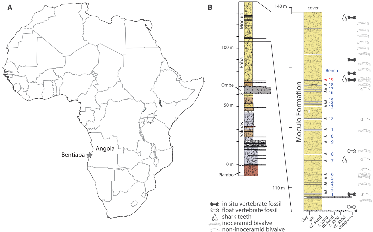
Fig. 1. A. Geographical location of the locality in Angola. B. Geological context and stratigraphic column with the position of Bench 19, the layer which produced the specimens described herein.
