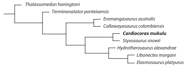
Fig. 4. Portion of recovered topology showing relationships of Cardiocrax mukulu . See text and Supplementary Material Figures 1 and 2 for detailed results.
