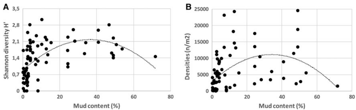
Fig. 17. Diversity (A; Shannon H' ; 2nd order polynomial, r^2 = 0.32 , P < 0.001 ) and density (B; total number per m^2 ; 2nd order polynomial, r^2 = 0.20 , P < 0.001 ) of macrozoobenthos with mud content (%DW).
