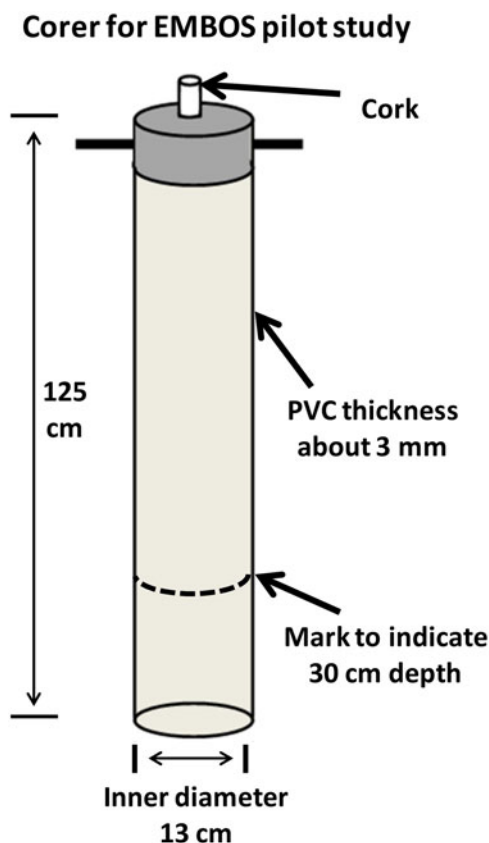
Fig. 3. Standard EMBOS sampling corer for soft sediments.
