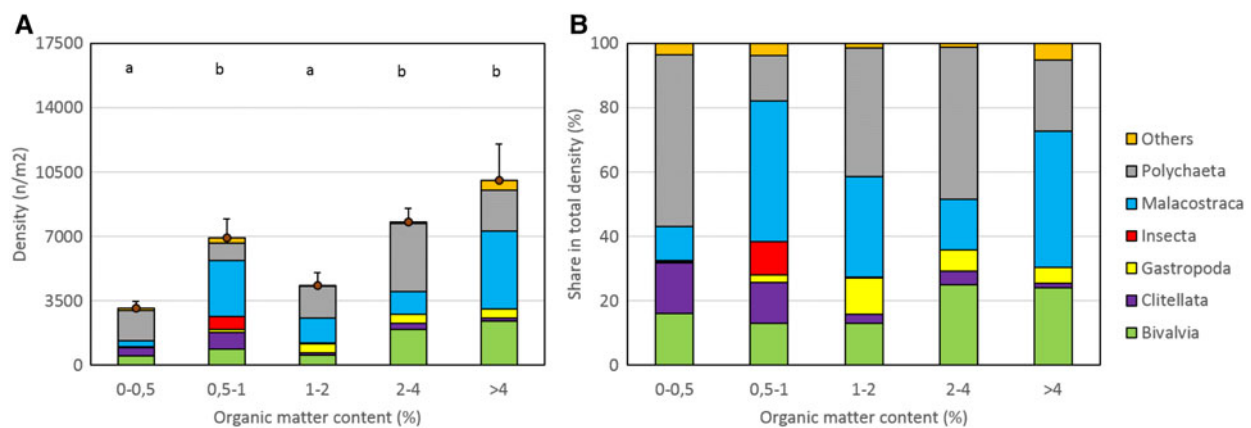
Fig. 9. Absolute (A) and relative (B) numbers of individuals per major taxonomic group with organic matter content (% DW). Average total densities \pm standard error for clusters of times 2 increasing organic matter contents; significant differences in total densities are indicated with different characters.
