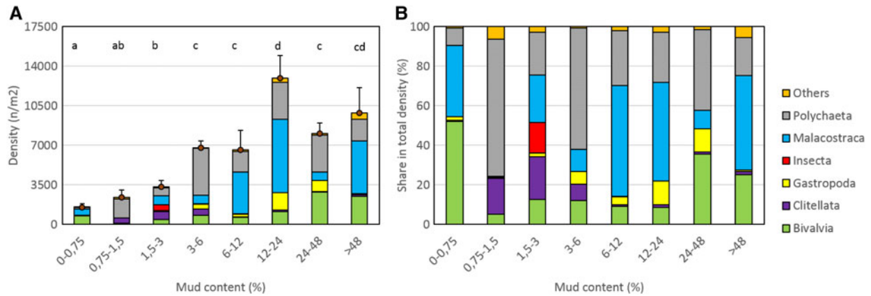
Fig. 8. Absolute (A) and relative (B) numbers of individuals per major taxonomic group with mud (<63 \mu\text{m} ) content (%). Average total densities \pm standard error for clusters of times 2 increasing mud contents; significant differences in total densities are indicated with different characters.
