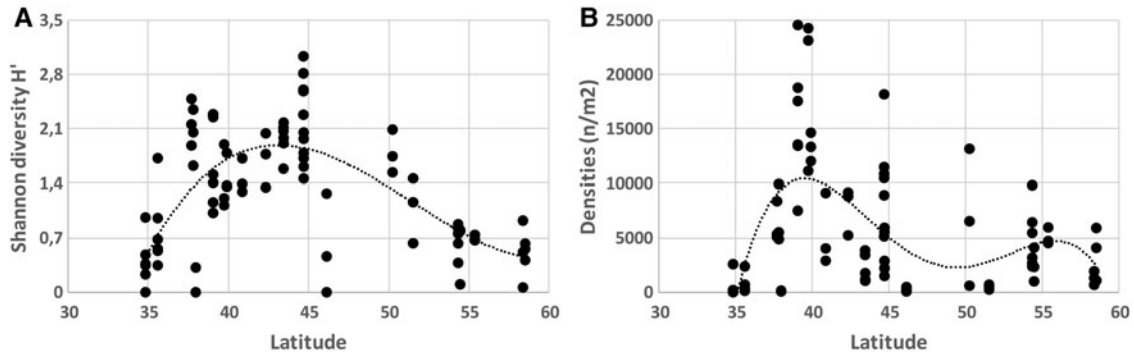
Fig. 14. Diversity (A; Shannon H' ; 3rd order polynomial, r^2 = 0.48 , P < 0.001 ) and density (B; total number per m^2 ; 4th order polynomial, r^2 = 0.34 , P < 0.001 ) of macrozoobenthos with latitude.
