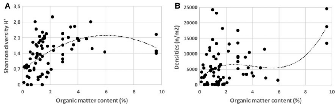
Fig. 18. Diversity (A; Shannon H' ; 2nd order polynomial, r^2 = 0.26 , P < 0.001 ) and density (B; total number per m^2 , 3rd order polynomial, r^2 = 0.21 , P < 0.001 ) of macrozoobenthos with organic matter content (%DW).
