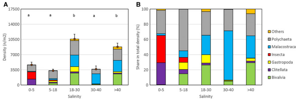
Fig. 6. Absolute (A) and relative (B) numbers of individuals per major taxonomic group with salinity. Average total densities \pm standard error for clusters according to the Thalassic salinity series (0–5 = oligohaline, 5–18 = mesohaline, 18–30 = polyhaline, 30–40 = mixoeuhaline, >40 = metahaline); significant differences in total densities are indicated with different characters.
