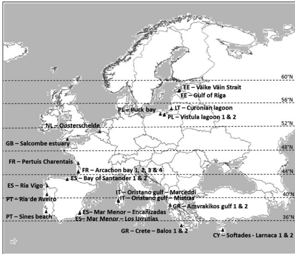
Fig. 1. EMBOS soft substrate sampling locations.
