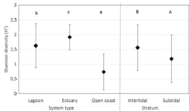
Fig. 13. Shannon diversity (average ± standard deviation) of macrozoobenthos for each of the identified system types and strata where sampling has taken place. Significant differences in Shannon diversity are indicated with different characters; both classification systems (types and strata) have been tested separately as they consist of the same samples.
