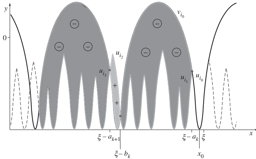
Figure 7. Illustration to estimate and compare the area between the graphs of u_{\text{flat}} and v_{i_0} .
