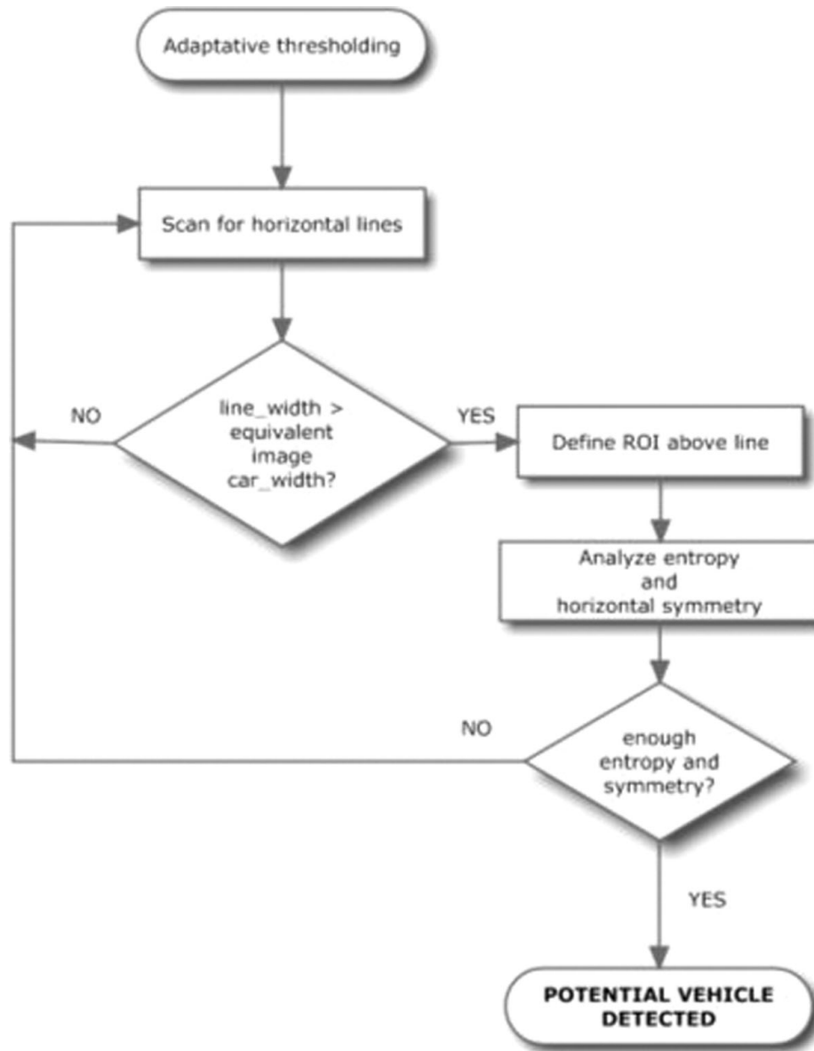
Fig. 6. Block diagram of the vehicle detection mechanism.
