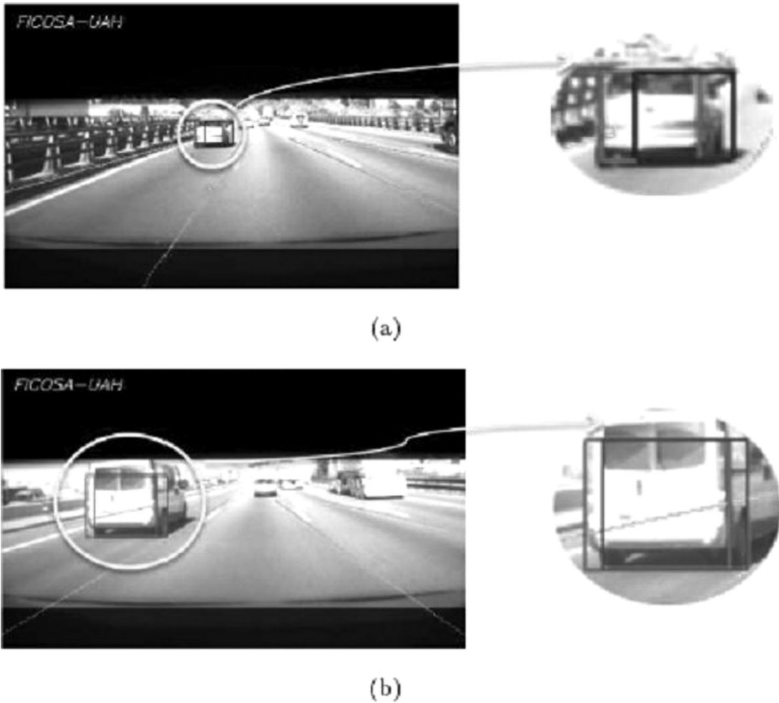
Fig. 8. Examples of symmetry-based vehicle position correction mechanism. Blue squares represent the original position of detected candidates. Red squares show the corrected position after symmetry analysis.
