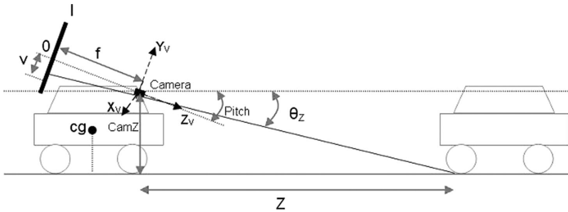
Fig. 5. Vertical road mapping geometry.
