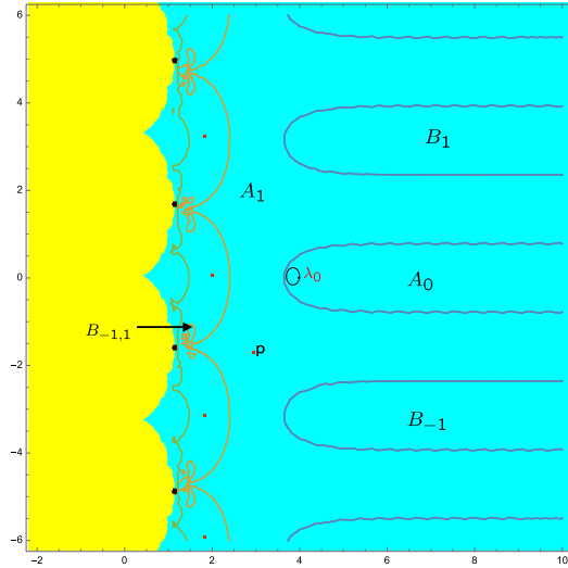
FIGURE 7. The ‘filled Julia set’ of Q(z) . The black dots are poles.
