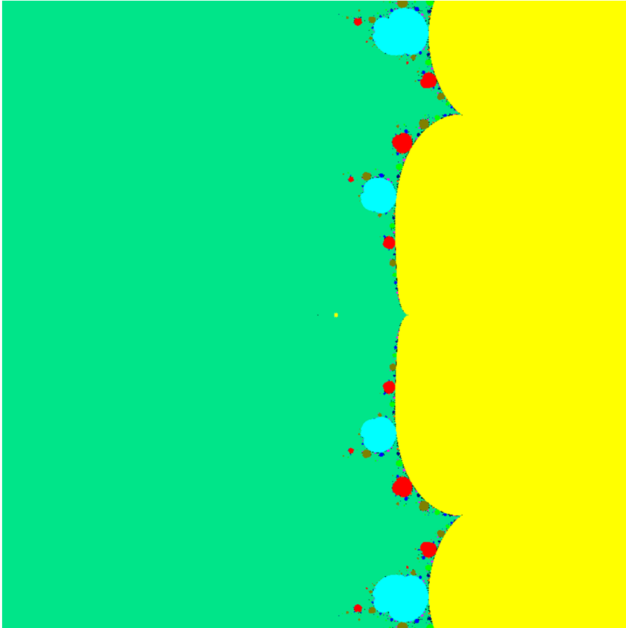
FIGURE 2. The \lambda plane divided into the shift locus and shell components. The large region on the left (green in the color version) is the shift locus \mathcal{S} . The region \mathcal{M}_\mu is the small disk inside it. The region \mathcal{M}_\lambda is on the right and shell components of different periods are shaded: the large region to the right is period 1; the biggest of the regions attached are period 2; the next smallest period 3, etc. Because \mathcal{M}_\mu is so small, only the period-1 region is visible.
