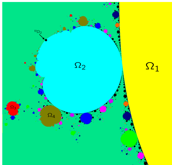
FIGURE 4. Blow-up of the \lambda plane near \mathcal{M}_\lambda with the periods labeled.
