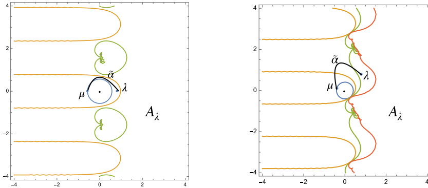
FIGURE 10. Two examples where the lifted curve is the one we need.
