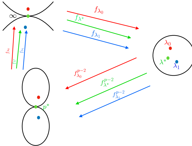
FIGURE 6. Transversality in the dynamic plane.
