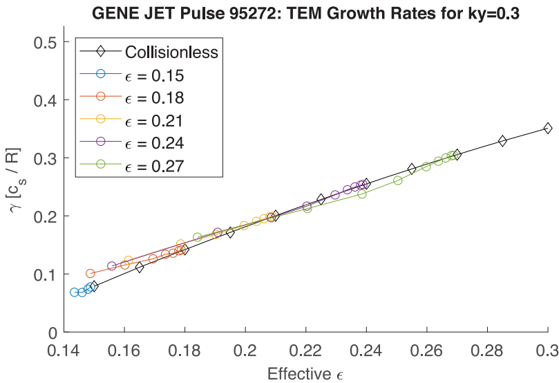
FIGURE 29. The TEM growth rates calculated by GENE for different values of nominal \epsilon plotted against effective \epsilon^* = (\pi \langle f_i^* \rangle / 2\sqrt{2})^2 using JET pulse 95 272 parameters where k_\theta \rho_s = 0.3 and \langle f_i^* \rangle is a function of \nu^* .
