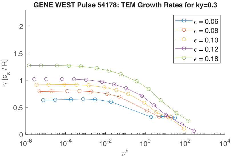
FIGURE 4. Collisional TEM growth rates calculated by GENE for different values of \epsilon plotted against \nu^* using WEST pulse 54178 parameters where k_\theta \rho_s = 0.3 . Note that the growth rate decreases nearly monotonically with \nu^* .
