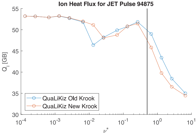
FIGURE 42. Total integrated ion heat flux calculated in QuaLiKiz for JET pulse 94 875 parameters plotted against \nu^* where \epsilon = 0.225 . Note that nominal \nu^* = 0.50 .
