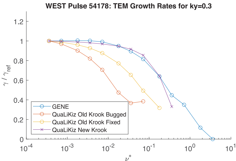
FIGURE 12. Collisional TEM growth rates calculated by GENE and QuaLiKiz (relative to their reference growth rates). Here, we use WEST pulse 54 178 parameters where k_\theta \rho_s = 0.3 and we plot against \nu^* for \epsilon = 0.10 .
