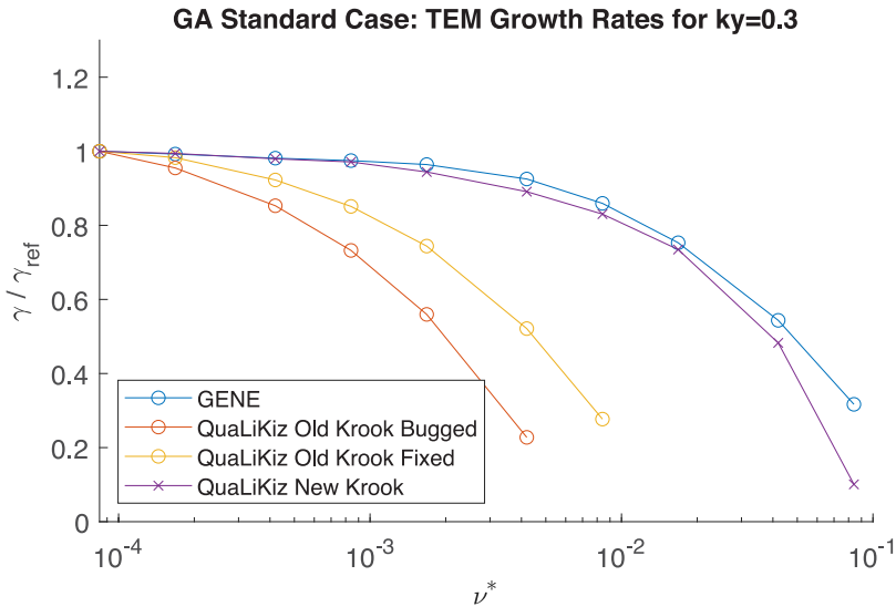
FIGURE 11. Collisional TEM growth rates calculated by GENE and QuaLiKiz (relative to their reference growth rates). Here, we use GA standard parameters where k_\theta \rho_s = 0.3 and we plot against \nu^* for \epsilon = 0.1667 .
