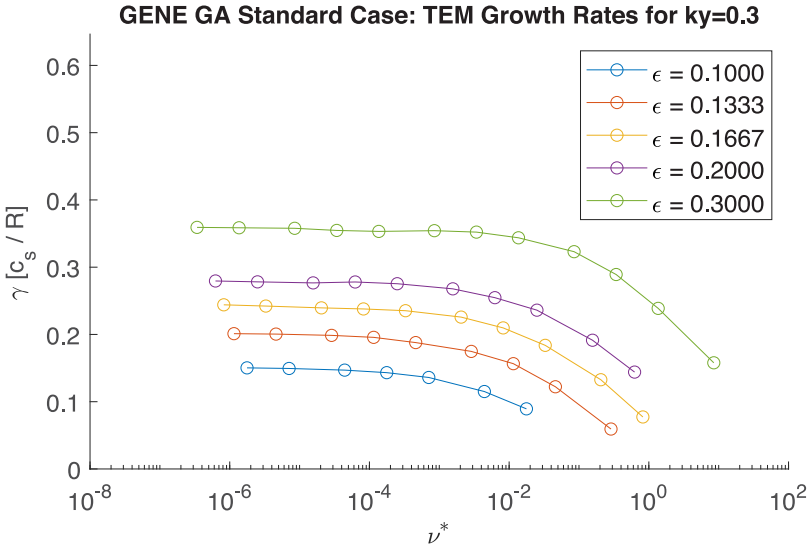
FIGURE 3. Collisional TEM growth rates calculated by GENE for different values of \epsilon plotted against \nu^* using GA standard parameters where k_\theta \rho_s = 0.3 . Note that the growth rate decreases nearly monotonically with \nu^* .
