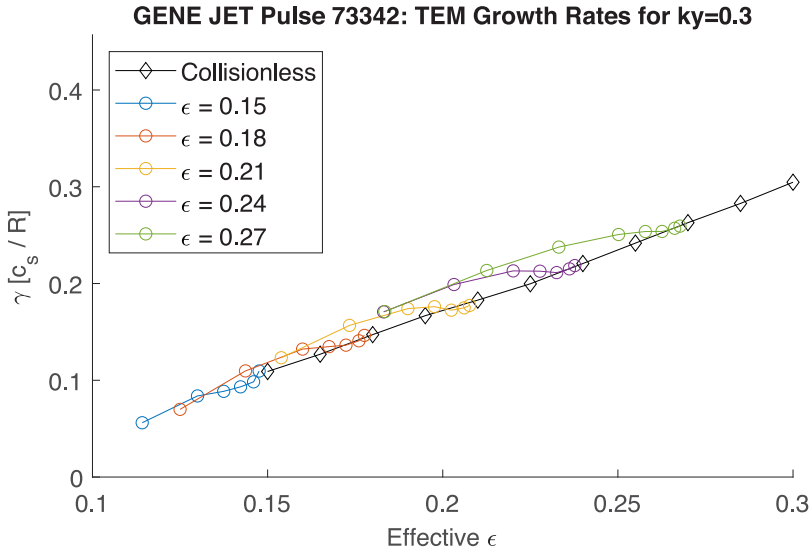
FIGURE 28. The TEM growth rates calculated by GENE for different values of nominal \epsilon plotted against effective \epsilon^* = (\pi \langle f_i^* \rangle / 2\sqrt{2})^2 using JET pulse 73 342 parameters where k_\theta \rho_s = 0.3 and \langle f_i^* \rangle is a function of \nu^* .
