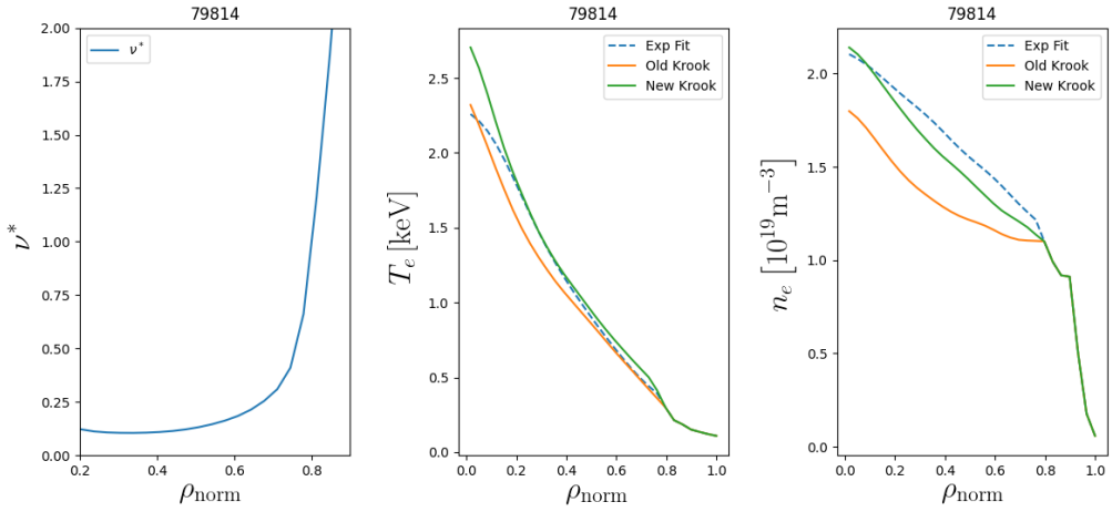
FIGURE 46. Integrated modelling of a JET L-mode case as part of collisionality scan in Tala et al. (2019).
