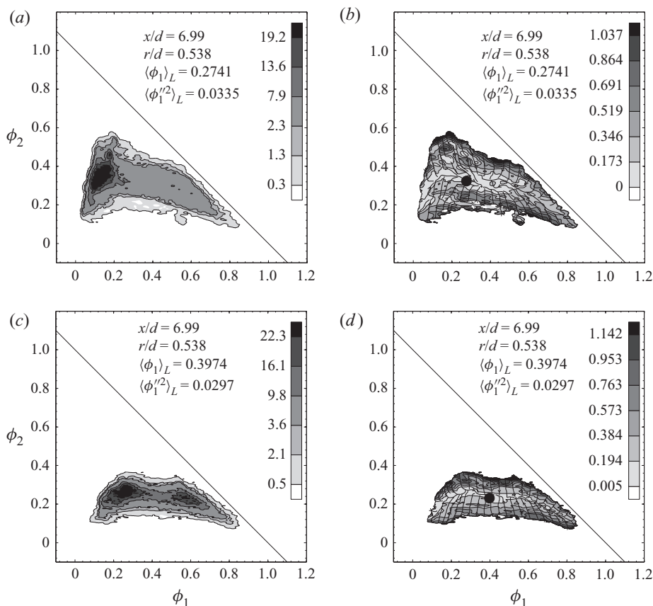
Figure 15. The j.j.d.f. (a,c) and conditionally filtered diffusion streamlines (b,d) conditional on the large SGS variance at x/d = 6.99 and r/d = 0.538 for Case I (a,b) and Case II (c,d).
