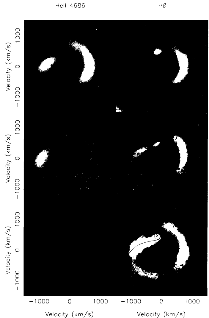
Fig. 1. Representative Doppler maps of WZ Sge in the light of HeII 4686Å (left) and H \beta on days 3 (top), 9 (middle) and 19 of the outburst.
