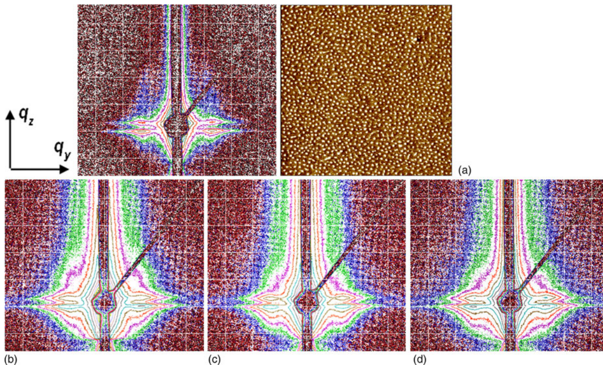
Figure 7. (Color online) GISAXS patterns of 40 nm thick films of sample PM70 after offline TEOS treatment (generation of SiO 2 NPs). (a) as coated, (b) after treatment with TEOS vapour, (c) after treatment with H 2 O/HCl vapour, (d) after annealing at 100 °C in vacuum. Scattering intensity plot (in miscolour) \log(I) vs. q_z, q_y ( q_z range: approx. 0.12–0.75 nm -1 , q_y range: approx. -0.36–0.36 nm -1 , mesh size \Delta q = 0.1 nm -1 ). Additionally in (a), an AFM phase contrast pattern is shown (pattern size 2 \times 2 \mu\text{m}^2 , scale 3°).
