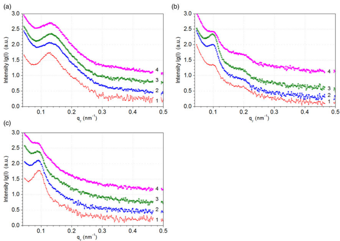
Figure 8. (Color online) Thin films of samples (a) PM70, (b) PM67, and (c) PM69: out-of-plane curves from GISAXS patterns at q_z = q_{y_{\text{oned},\text{BCP}}} after offline TEOS treatment [(1) as coated, (2) after treatment with TEOS vapour, (3) after treatment with H 2 O/HCl vapour, (4) annealed at 100 °C in vacuum], curves are shifted vertically for clarity. Corresponding 2D GISAXS patterns are given in Figures 7(a)–7(d) at the example of sample PM70.
