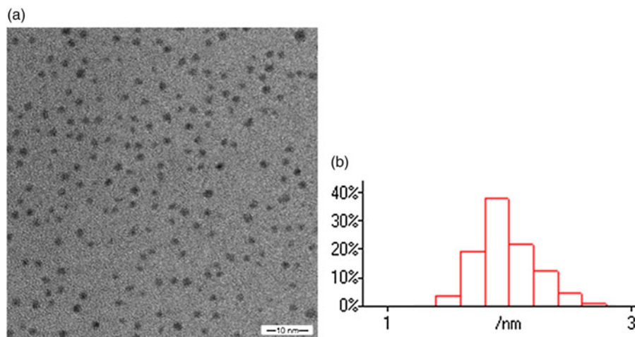
Figure 2. (Color online) (a) TEM image (magnification: 400 000 \times , scale bar: 10 nm) and (b) NP size distribution of dodecanthiol-stabilized Au NPs (Au18) with mean core diameter of 2 nm.
