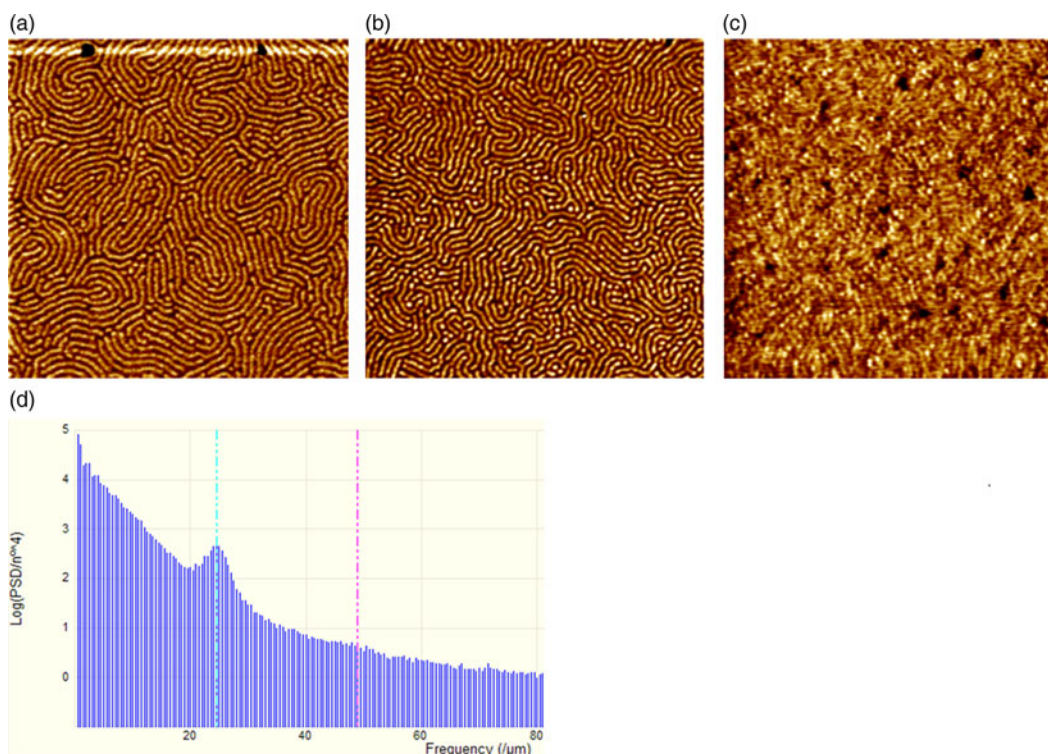
Figure 5. (Color online) AFM results from 20 nm films of sample PM13/Au18 vs. concentration of NPs [(a–c): 0, 1, and 5 wt.%; as spin-coated]. AFM phase contrast images (pattern size 2 \times 2\ \mu\text{m}^2 , scale 3^\circ ); (d) PSD of FFT image of AFM image (a) ( L_0 is the result from reading of the peak position).
