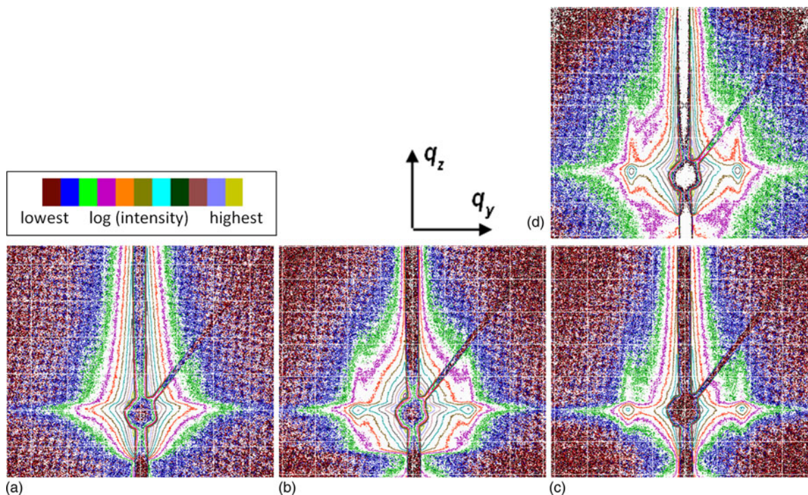
Figure 4. (Color online) 20 nm films of sample PM13/Au18 vs. concentration of NPs [(a–d): 0, 1, 5, and 5 wt.%] and influence of SVA with THF [(a–c) as spin-coated, (d) vapour-annealed]. GISAXS pattern, scattering intensity plot (in miscolour) \log(I) vs. q_z , q_y ( q_z range: approx. 0.08\text{--}0.78\text{ nm}^{-1} , q_y range: approx. -0.40\text{--}0.40\text{ nm}^{-1} , mesh size \Delta q = 0.1\text{ nm}^{-1} ).
