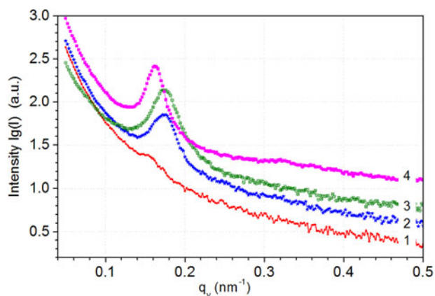
Figure 6. (Color online) GISAXS results from 20 nm films of sample PM13/Au18 vs. concentration of NPs [(1–3): 0, 1, and 5 wt.%] and influence of SVA with THF (4) for film with 5 wt.% Au NPs]. Out-of-plane curves from the GISAXS patterns [Figures 4(a)–4(d)], taken at q_z = q_{Y_{\text{oned}}, \text{BCP}} .
