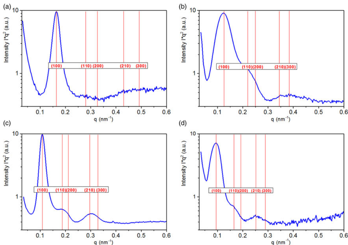
Figure 3. (Color online) Lorentz-corrected SAXS curves of corresponding BCP bulk material with hexagonal packed cylinder morphologies [with Miller indexing of the first reflections ( hk0 )]. (a) PM13, (b) PM70, (c) PM67, and (d) PM69.
