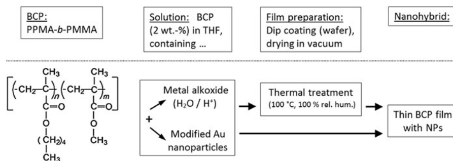
Figure 1. Schematic representation of the steps for achieving block copolymer/NP hybrids with PPMA- b -PMMA block copolymers in both applied preparation procedures.
