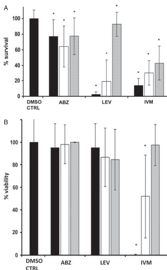
Fig 1. Anthelmintic activity of albendazole, levamisole and ivermectin against Ancylostoma ceylanicum L3 (A) and adult worms (B). The percentage survival or the viability scores are expressed as percentage of the controls. DMSO CTRL = DMSO control, ABZ = albendazole, LEV = levamisole, IVM = ivermectin. Black bars show 100 \mu g/ml; white bars show 10 \mu g/ml; striped bars show 1 \mu g/ml. The assays were conducted at least twice in triplicates. * p \leq 0.05 (A: Fisher's exact test; B: Mann-Whitney U test).
