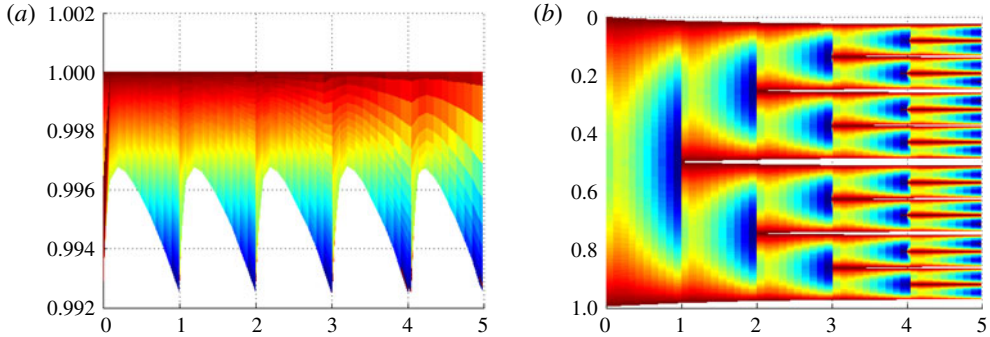
FIGURE 6. (Colour online) Demonstration of the fractal-forming behaviour for the supercritical conditions given in equation (3.27). Panel (a) shows minimum concentration (lower bound) and concentration profiles (colours), while (b) shows the concentration (colours) plotted on the domains as they split, thus white represents ice. For both panels, time is given with respect to the transformed time \eta .
