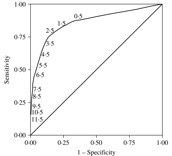
Fig. 1. Receiver operating characteristic (ROC) curve of the GHQ.
