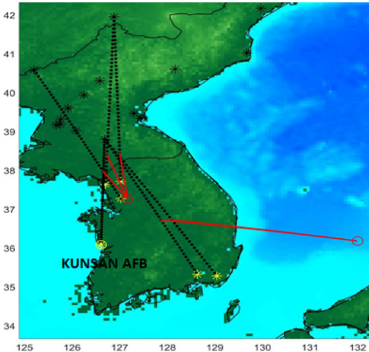
FIGURE 2 Performance of South Korean PATRIOT, THAAD, and Aegis BMD (against lofted trajectories)
