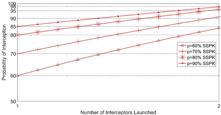
FIGURE 4 Impact of Interceptor SSPK on Probability of Interception
