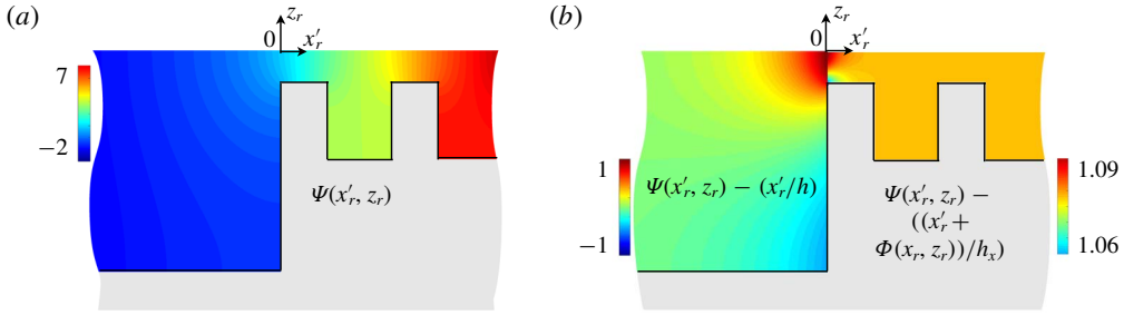
FIGURE 7. (Colour online) (a) Example of field \Psi(x'_r, z_r) satisfying the elementary problem (4.17). (b) Illustration of the extension of transition effects due to an evanescent field, with a resulting coefficient \mathcal{B} = 1.08 in (4.18).
