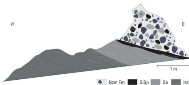
Figure 1. (Colour online) Schematic diagram showing lithological contact at Idhen, UAE. The silicified serpentinite (SiSp, black colour) overlies serpentinite (Sp) and harzburgite (Hzb). All units are cross-cut by an irregular array of carbonate- and chalcedony-dominated veins (modified from Lacinska et al. 2014).
