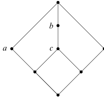
FIGURE 1. A pseudocomplemented semilattice.
