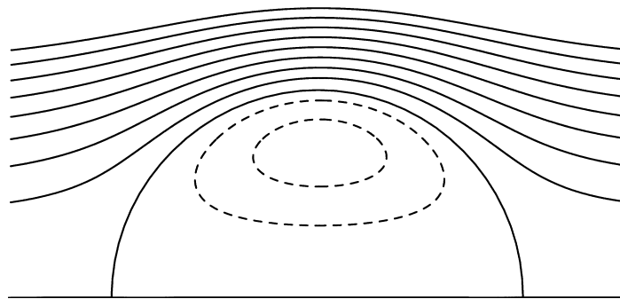
FIGURE 2. Streamlines of the first approximation to the flow: \bar{\psi}_0 (solid) outside the sphere, \bar{\psi}_1 (dashed) inside it.
