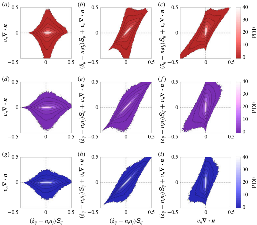
FIGURE 6. Joint PDFs of (\delta_{ij} - n_i n_j) S_{ij} , v_n \nabla \cdot n and their sum for Ri0 (a-c), Ri11 (d-f) and Ri22 (g-h) for 30 < t < 120 . The corresponding values of the black contour lines increase with logarithmic intervals.
