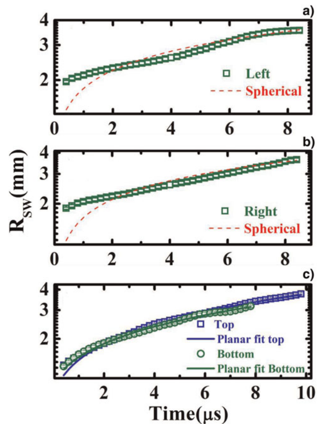
Fig. 7. (Color online) (a) Left and (b) Right SW location data showing radius of curvature of shock front ( R_{SW} ) along the horizontal direction at 75 mJ input laser energy. Solid lines in the figure are the curve fit to Taylor solution for spherical shock wave. (c) Radius of curvature of shock front ( R_{SW} ) along the vertical direction at 75 mJ input laser energy. Solid lines in the figure are the curve fit to Taylor solution for planar shock wave.
