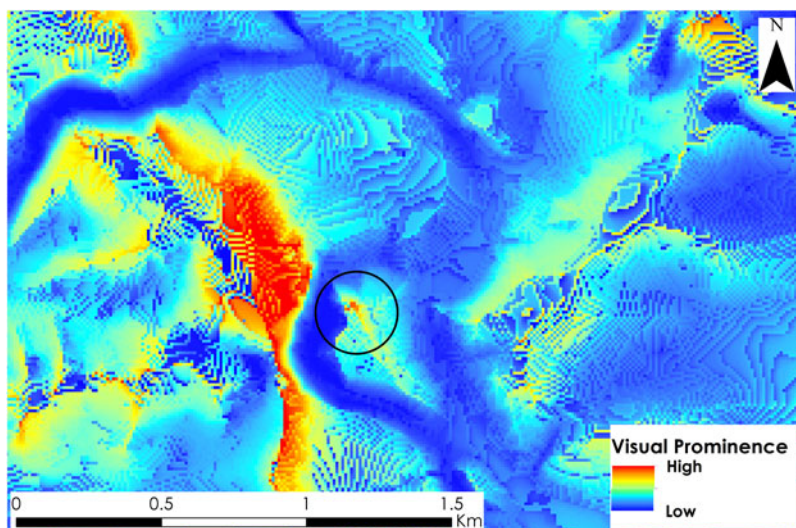
Figure 5. Total viewshed derived from a 10 m-resolution DTM. The cliffs to the west of Dinas Powys are visually prominent but not readily defensible and are difficult to access from natural routeways crossing lower ground. Dinas Powys is located within the centre of the black circle.
