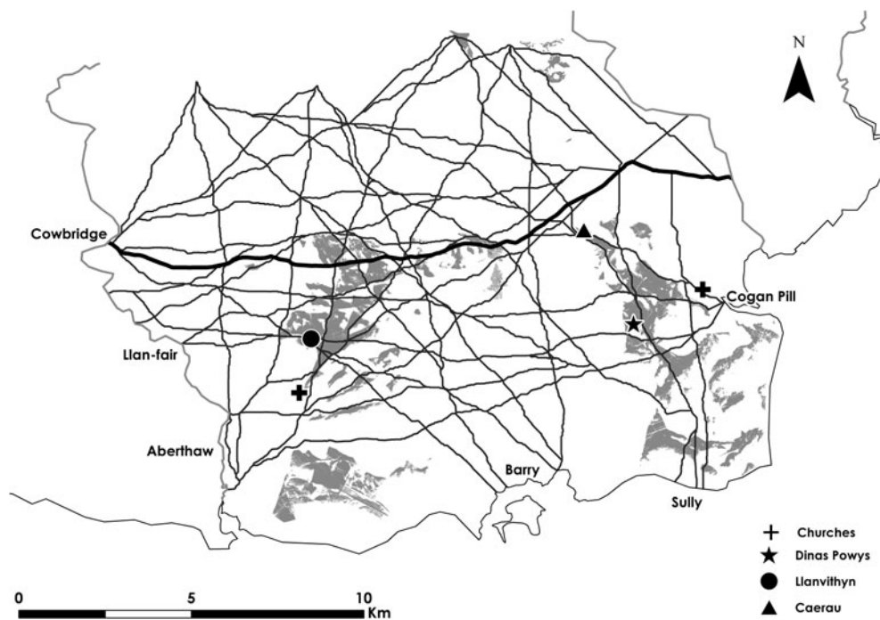
Figure 3. The network of LCPs with viewsheds from Dinas Powys and Llanvethin (in grey). Entry/exit nodes referred to in the text are labelled. The Roman road is highlighted.
