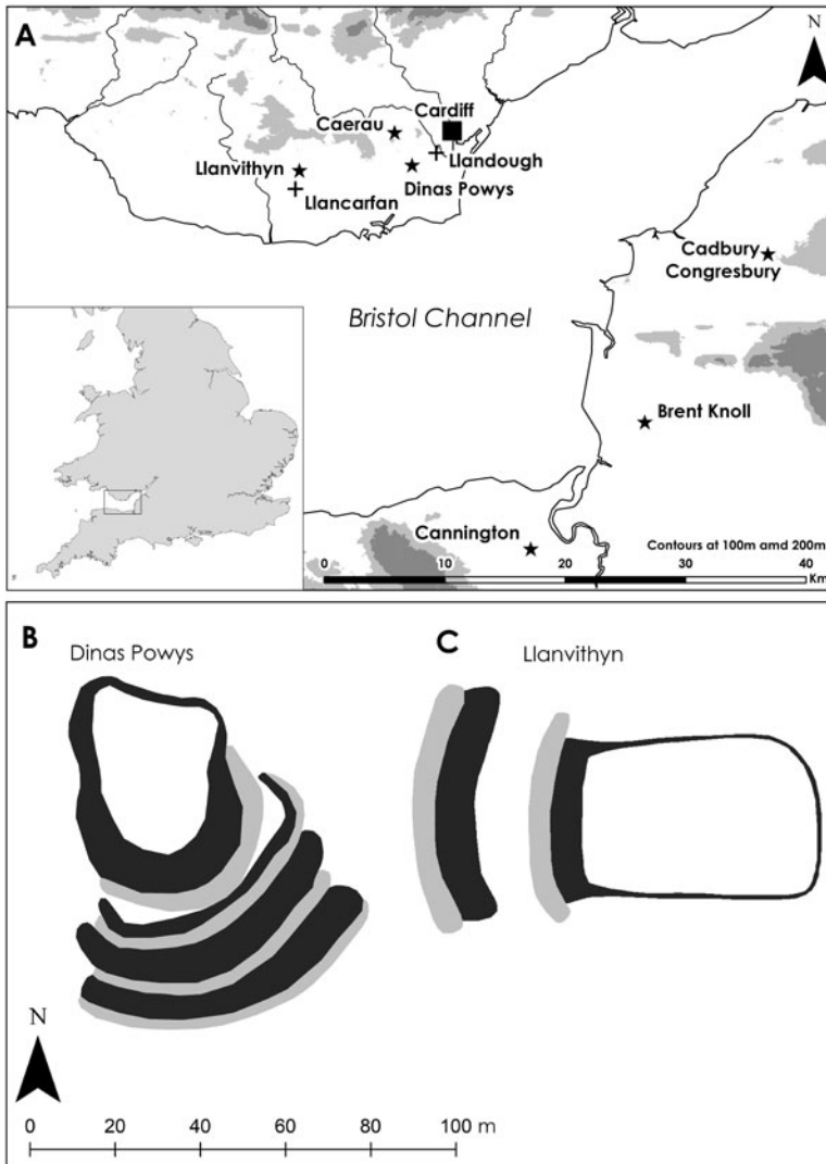
Figure 1. Location map and site plans. B: Dinas Powys: after Alcock, 1963, based on survey by RCAHMW, with additions. C: Llanvithyn. Banks in dark grey, ditches in light grey. © Crown Copyright and Database Right (June 2019) OS (Digimap Licence).
