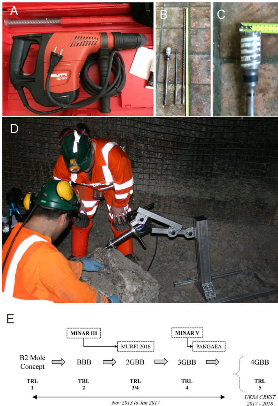
Fig. 4. Some of the sample acquisition instrumentation deployed in MINAR 5. (a)–(c) NASA drill. (a) The Hilti Drill TE 50, 1050 Watts; (b) 42 cm core string; 40.6 cm cutting string; 92.7 cm cuttings string; (c) core drill bit diameter 5 and 7 cm long, (d) The SPLIT instrument in operation on an artificial outcrop of halite in the Mars Yard; (e) the use of MINAR for the methodical development of the SPLIT technology (see ‘Results’ section for details).
