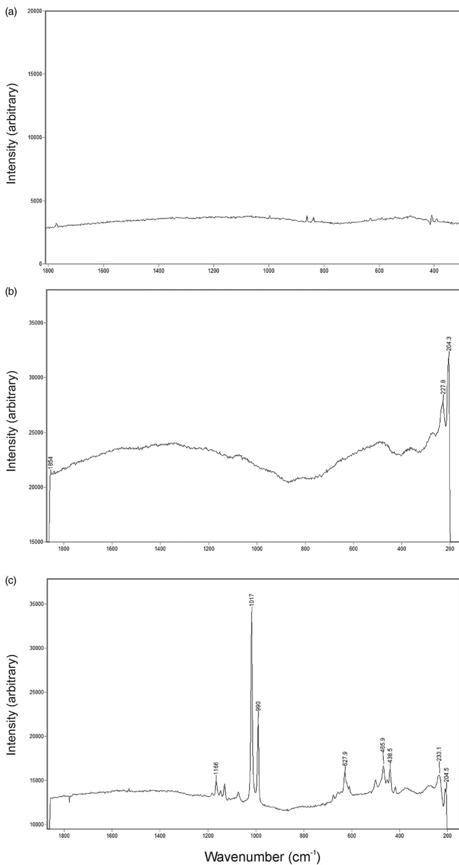
Fig. 11. Raman spectroscopy. Spectral plots of (a) halite, (b) iron oxide/clay inclusions in potash, (c) polyhalite.
