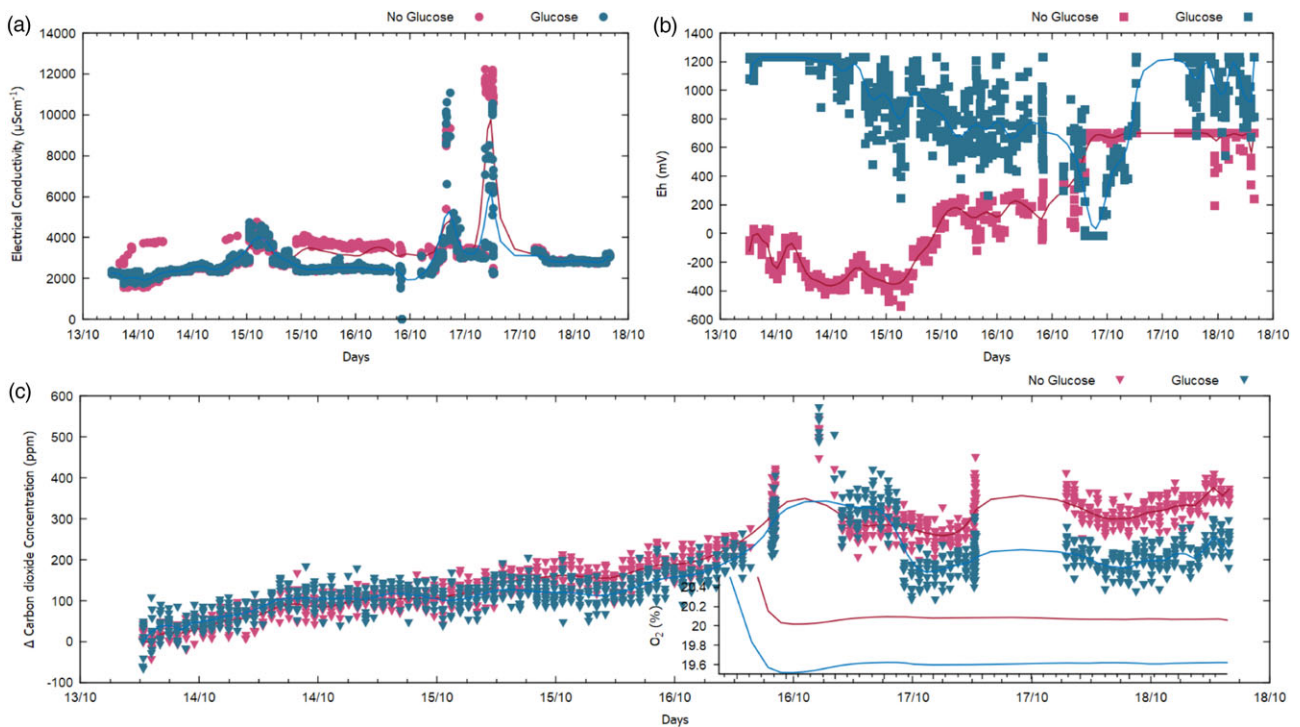
Fig. 13. Metabolt operation. (a) Comparison of electrical conductivity in samples with and without glucose. (b) Comparison of redox potential (Eh) in samples with and without glucose. (c) Comparison of change in carbon dioxide levels in samples with and without glucose; (inset) anti-correlation with oxygen levels.
