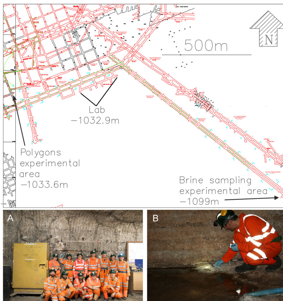
Fig. 2. Sites where samples were acquired and studied during MINAR 5 in relation to the underground laboratory and mine roadways (top). The 'Lab' constitutes the underground laboratory and Mars Yard (see Fig. 1). Depths below sea level are shown. (a) Polygons experimental area. The dark lineations of the polygons can be seen in the wall behind the sampling team. (b) Brine sampling experimental area. ESA astronaut Matthias Maurer samples brine solutions at the edge of the pool.
