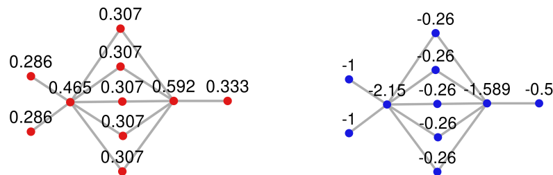
Figure 7: Normalized curvature \mathcal{K}_{G,\cdot}^{\text{nor}}(\infty) Figure 8: Non-normalized curvature \mathcal{K}_{G,\cdot}(\infty)
