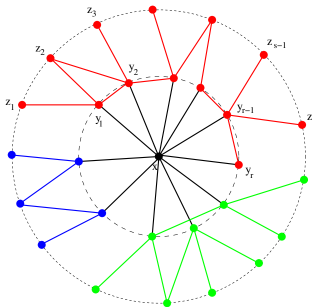
Figure 5: Connected components of \mathring{B}_2(x) in different colours; choosing the red connected component leads to d = 11 and r = 6 .
