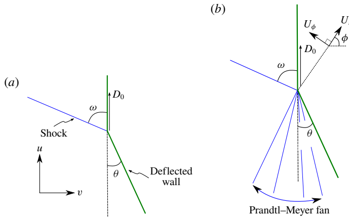
FIGURE 4. Shock polar analysis for (a) strong confinement and (b) weak confinement configurations.
