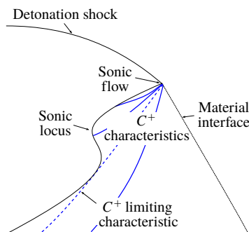
FIGURE 2. Schematic of C^+ characteristics for weak confinement originating from the expansion fan centred at the intersection of the detonation shock and sonic locus and impinging on the sonic locus. Based on a schematic shown in Bdzil (1981).
